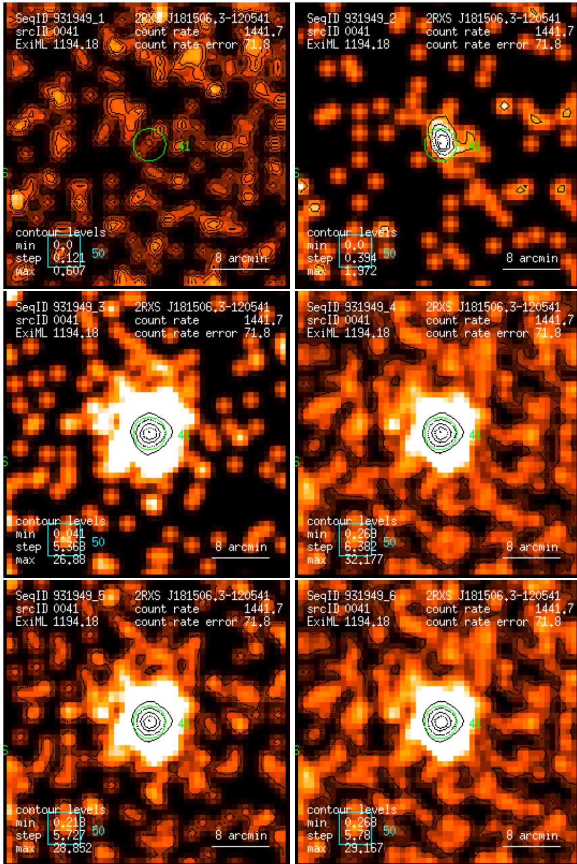
Figure 41: RASS 931949: detection 0041: band rate images, Gaussian filter: (1) PSPC channels 11 – 41, (2) 52 – 90, (3) 91 – 201, (4) 11 – 235, (5) 52 – 201, (6) 11 – 201. Broad band rates in counts/ks. Band rate contour levels in counts/ks/arcmin 2 .
