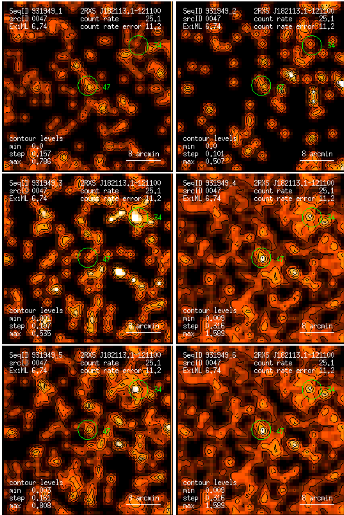
Figure 47: RASS 931949: detection 0047: band rate images, Gaussian filter: (1) PSPC channels 11 – 41, (2) 52 – 90, (3) 91 – 201, (4) 11 – 235, (5) 52 – 201, (6) 11 – 201. Broad band rates in counts/ks. Band rate contour levels in counts/ks/arcmin 2 .
