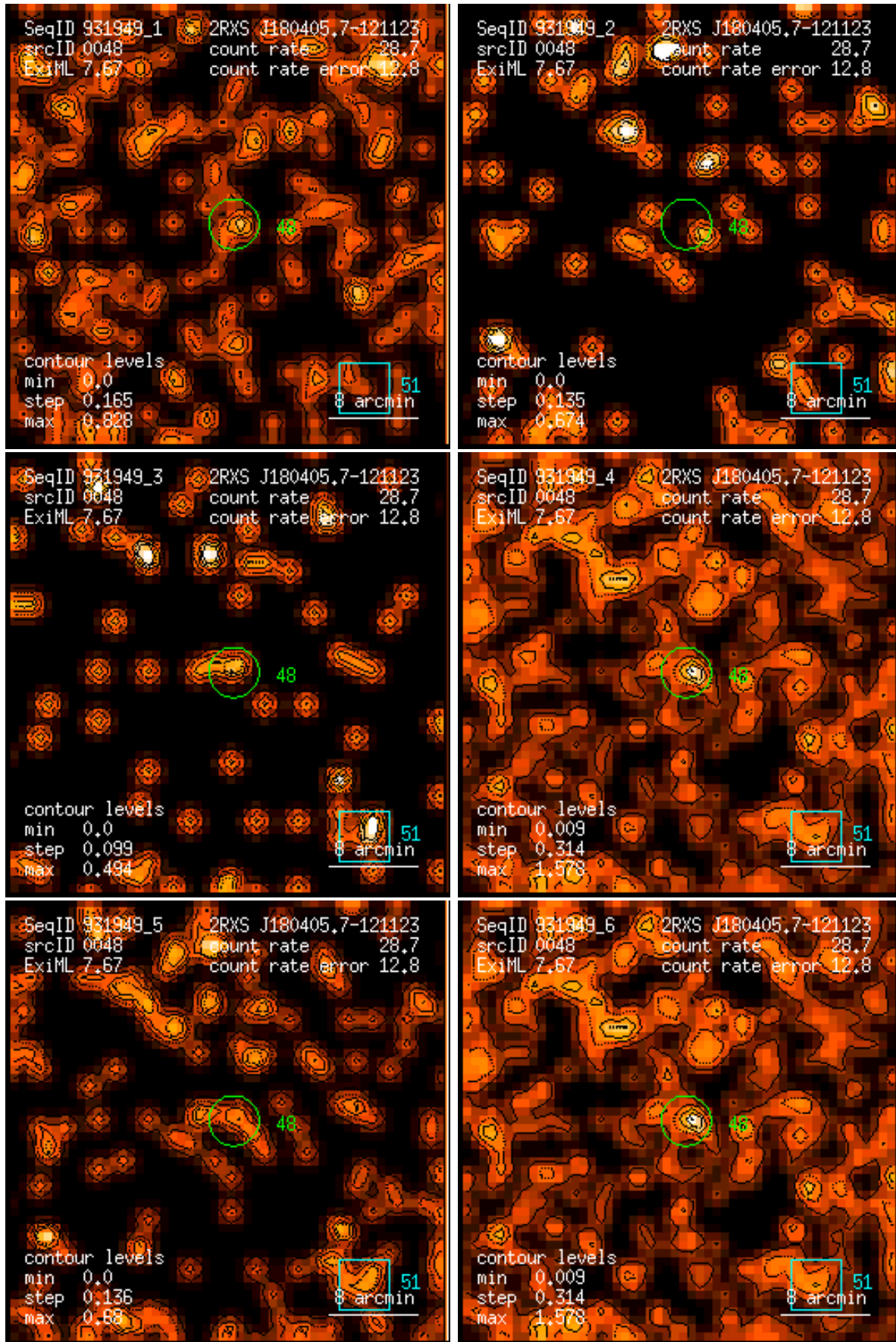
Figure 48: RASS 931949: detection 0048: band rate images, Gaussian filter: (1) PSPC channels 11 – 41, (2) 52 – 90, (3) 91 – 201, (4) 11 – 235, (5) 52 – 201, (6) 11 – 201. Broad band rates in counts/ks. Band rate contour levels in counts/ks/arcmin 2 .
