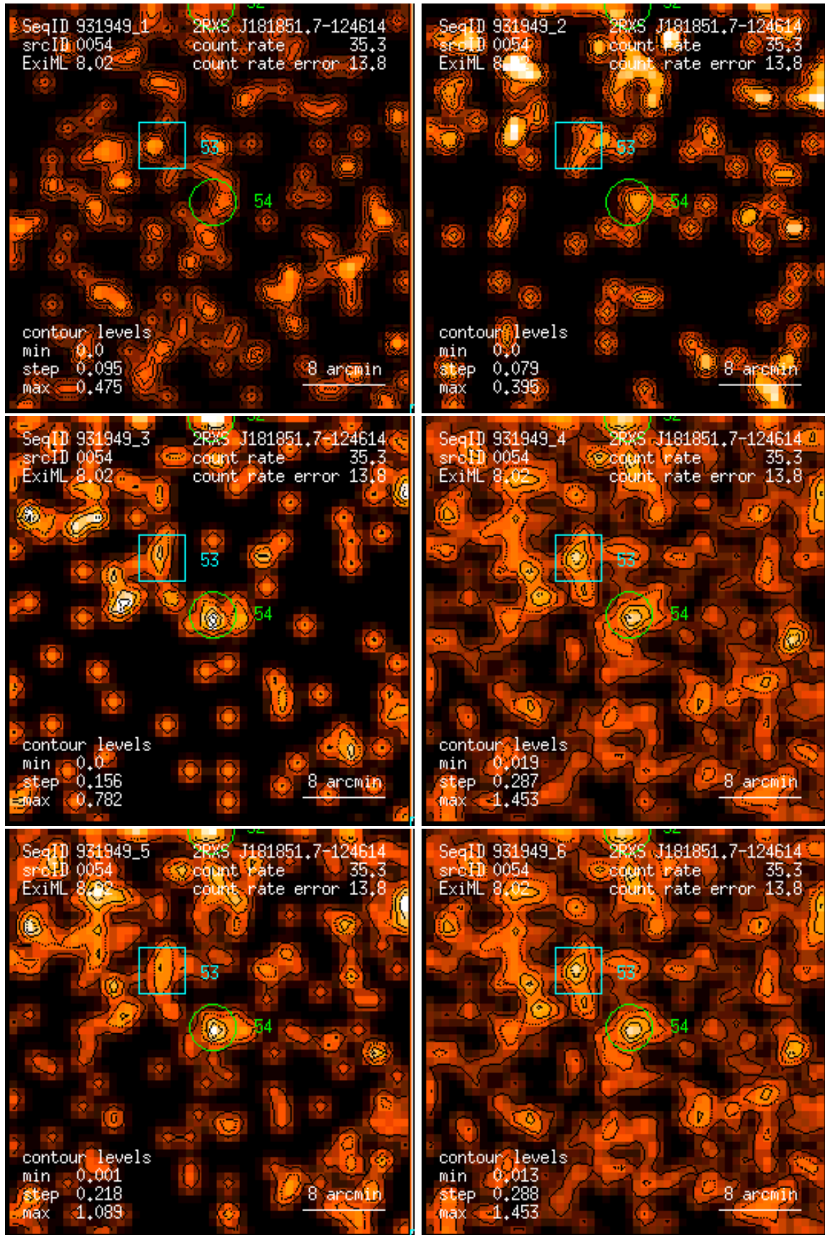
Figure 54: RASS 931949: detection 0054: band rate images, Gaussian filter: (1) PSPC channels 11 – 41, (2) 52 – 90, (3) 91 – 201, (4) 11 – 235, (5) 52 – 201, (6) 11 – 201. Broad band rates in counts/ks. Band rate contour levels in counts/ks/arcmin 2 .
