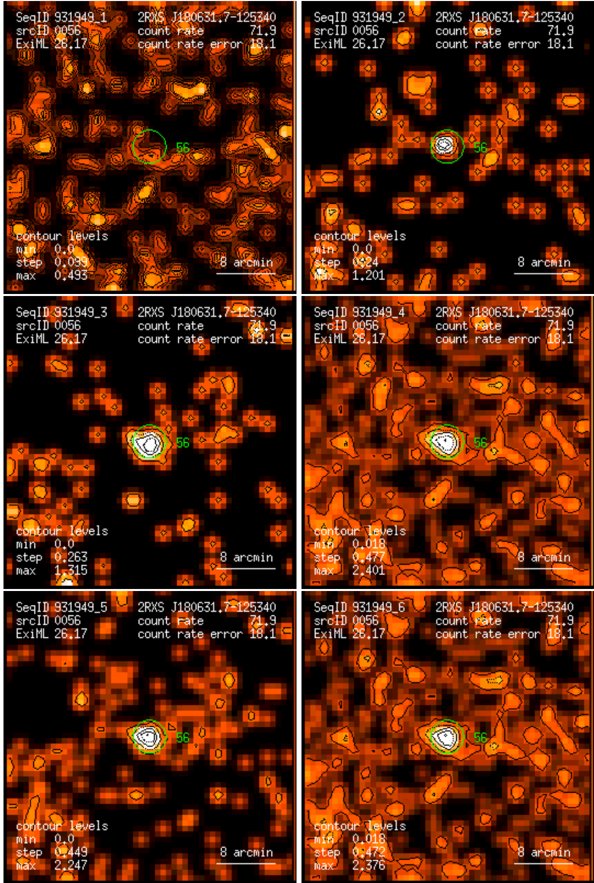
Figure 56: RASS 931949: detection 0056: band rate images, Gaussian filter: (1) PSPC channels 11 – 41, (2) 52 – 90, (3) 91 – 201, (4) 11 – 235, (5) 52 – 201, (6) 11 – 201. Broad band rates in counts/ks. Band rate contour levels in counts/ks/arcmin 2 .
