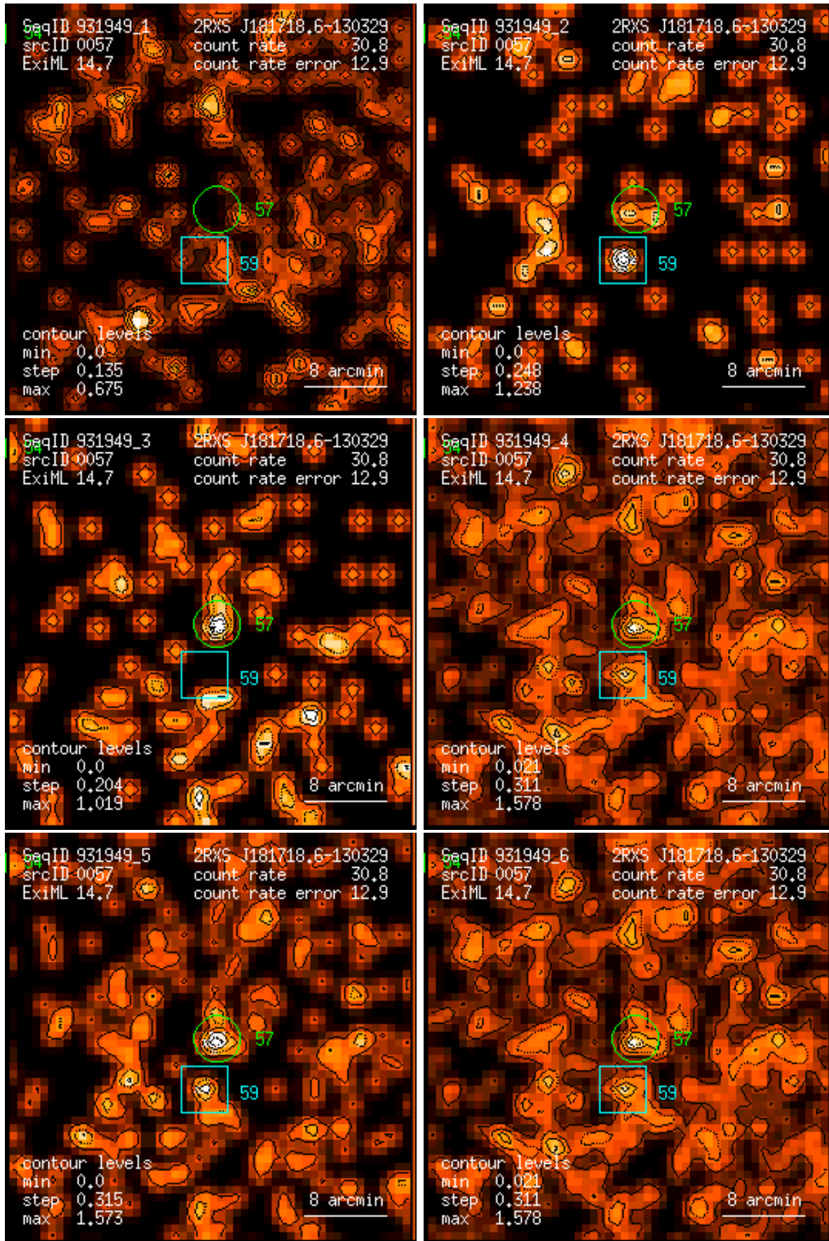
Figure 57: RASS 931949: detection 0057: band rate images, Gaussian filter: (1) PSPC channels 11 – 41, (2) 52 – 90, (3) 91 – 201, (4) 11 – 235, (5) 52 – 201, (6) 11 – 201. Broad band rates in counts/ks. Band rate contour levels in counts/ks/arcmin 2 .
