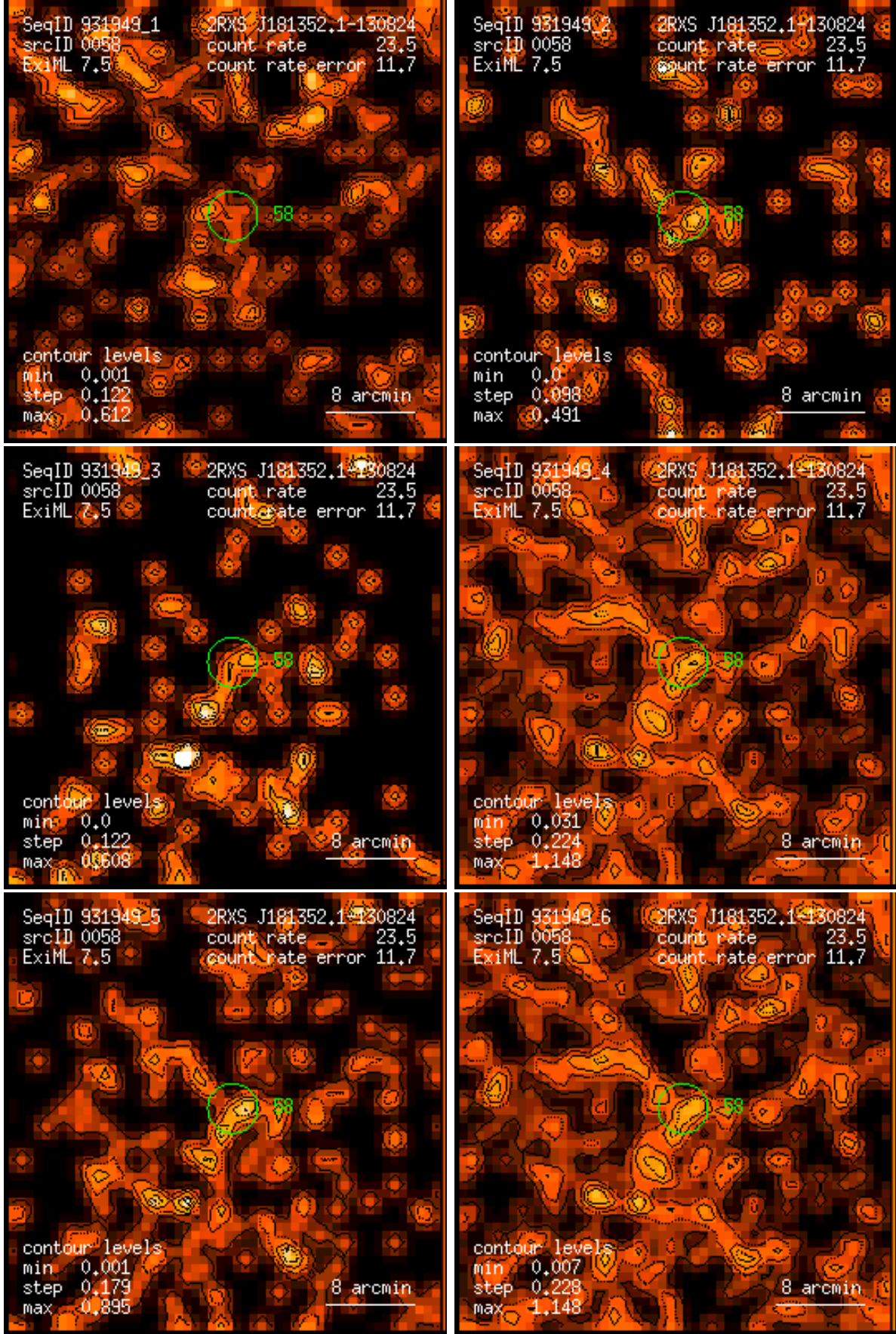
Figure 58: RASS 931949: detection 0058: band rate images, Gaussian filter: (1) PSPC channels 11 – 41, (2) 52 – 90, (3) 91 – 201, (4) 11 – 235, (5) 52 – 201, (6) 11 – 201. Broad band rates in counts/ks. Band rate contour levels in counts/ks/arcmin 2 .
