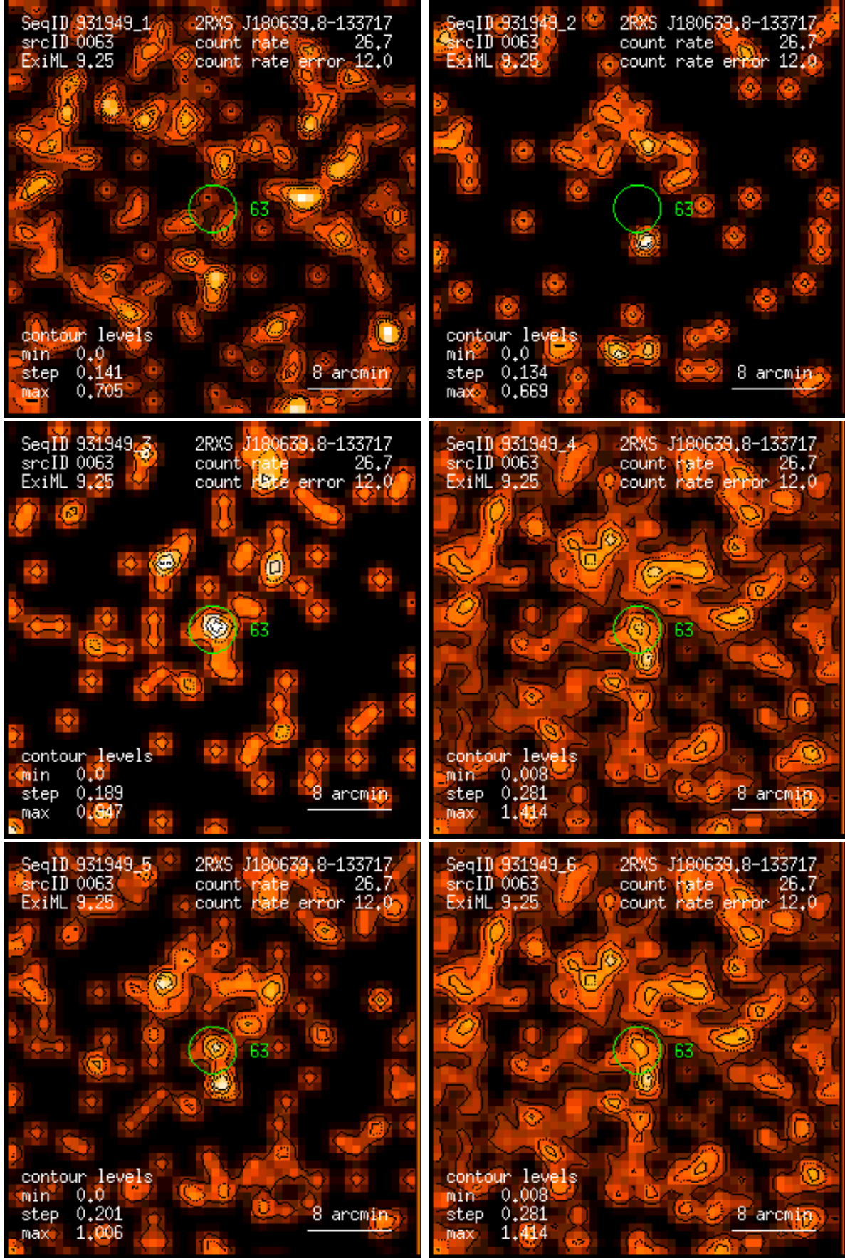
Figure 63: RASS 931949: detection 0063: band rate images, Gaussian filter: (1) PSPC channels 11 – 41, (2) 52 – 90, (3) 91 – 201, (4) 11 – 235, (5) 52 – 201, (6) 11 – 201. Broad band rates in counts/ks. Band rate contour levels in counts/ks/arcmin 2 .
