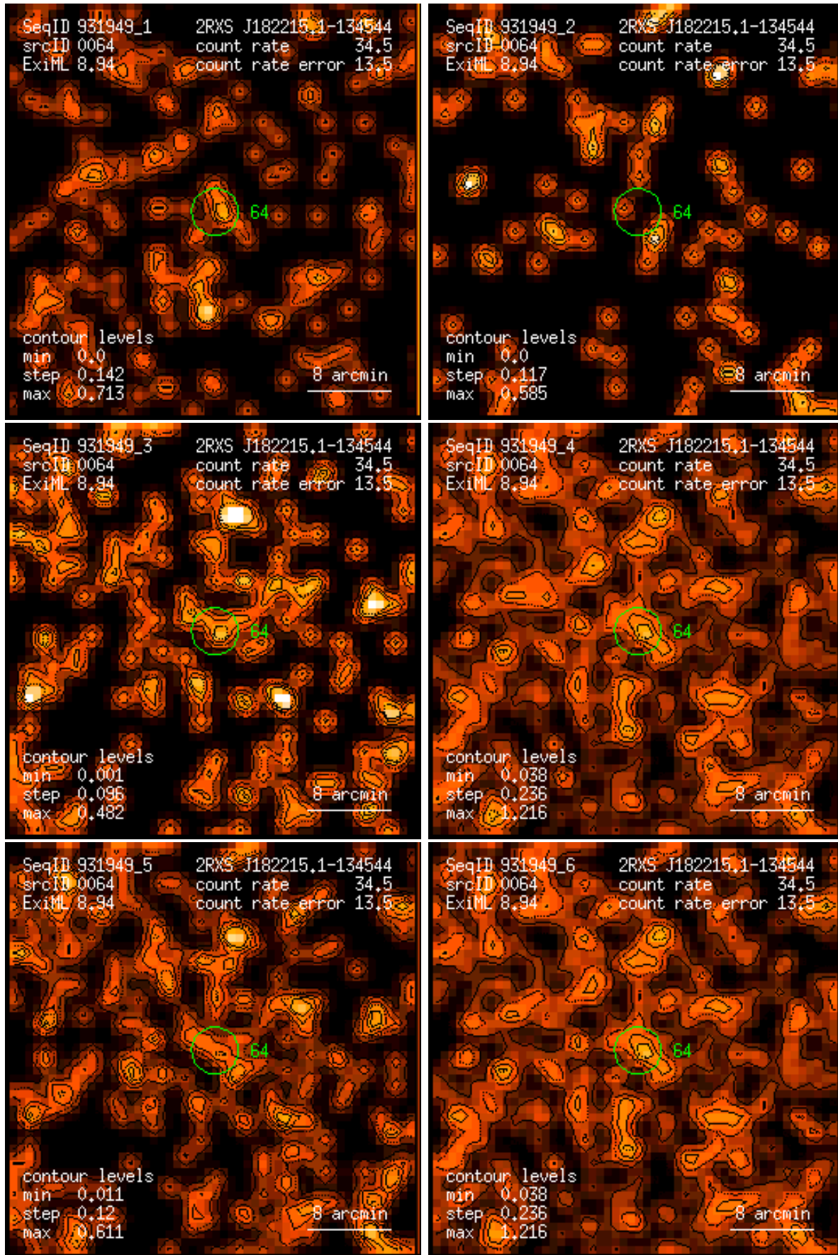
Figure 64: RASS 931949: detection 0064: band rate images, Gaussian filter: (1) PSPC channels 11 – 41, (2) 52 – 90, (3) 91 – 201, (4) 11 – 235, (5) 52 – 201, (6) 11 – 201. Broad band rates in counts/ks. Band rate contour levels in counts/ks/arcmin 2 .
