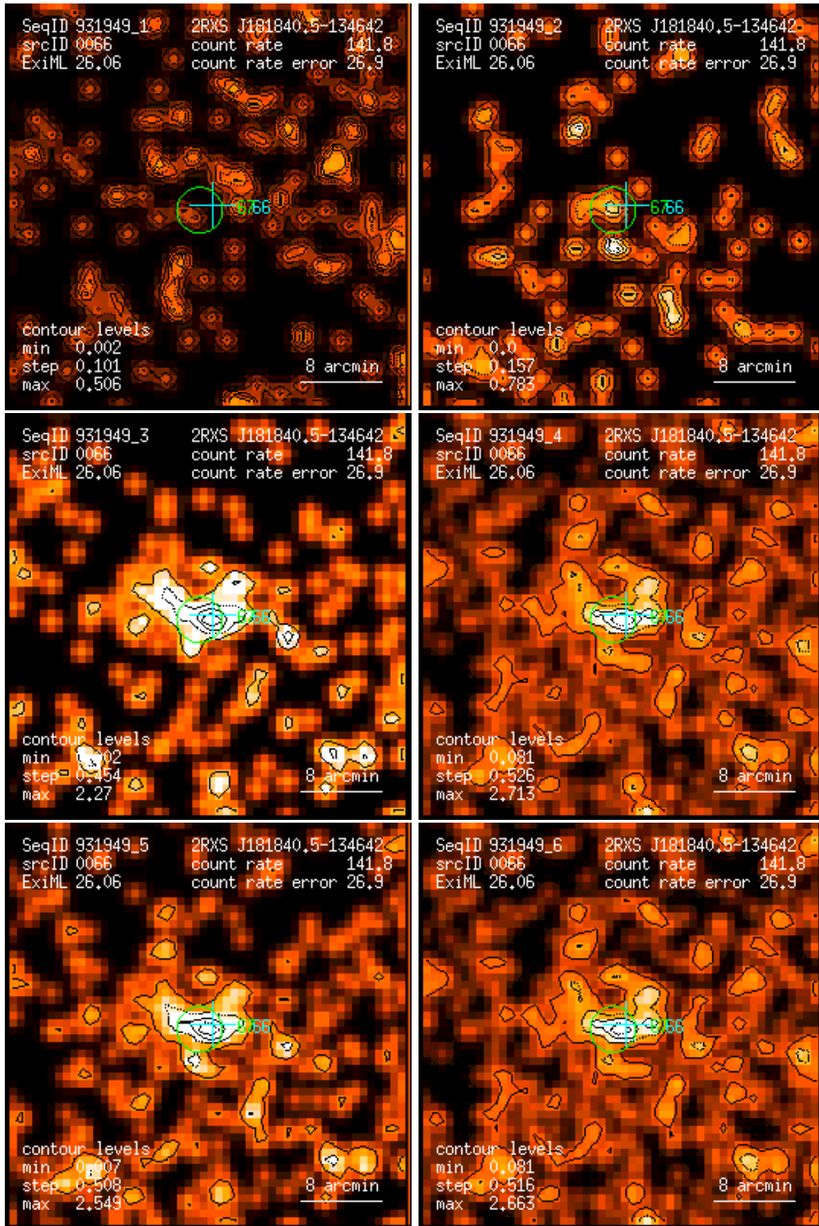
Figure 66: RASS 931949: detection 0066: band rate images, Gaussian filter: (1) PSPC channels 11 – 41, (2) 52 – 90, (3) 91 – 201, (4) 11 – 235, (5) 52 – 201, (6) 11 – 201. Broad band rates in counts/ks. Band rate contour levels in counts/ks/arcmin 2 .
