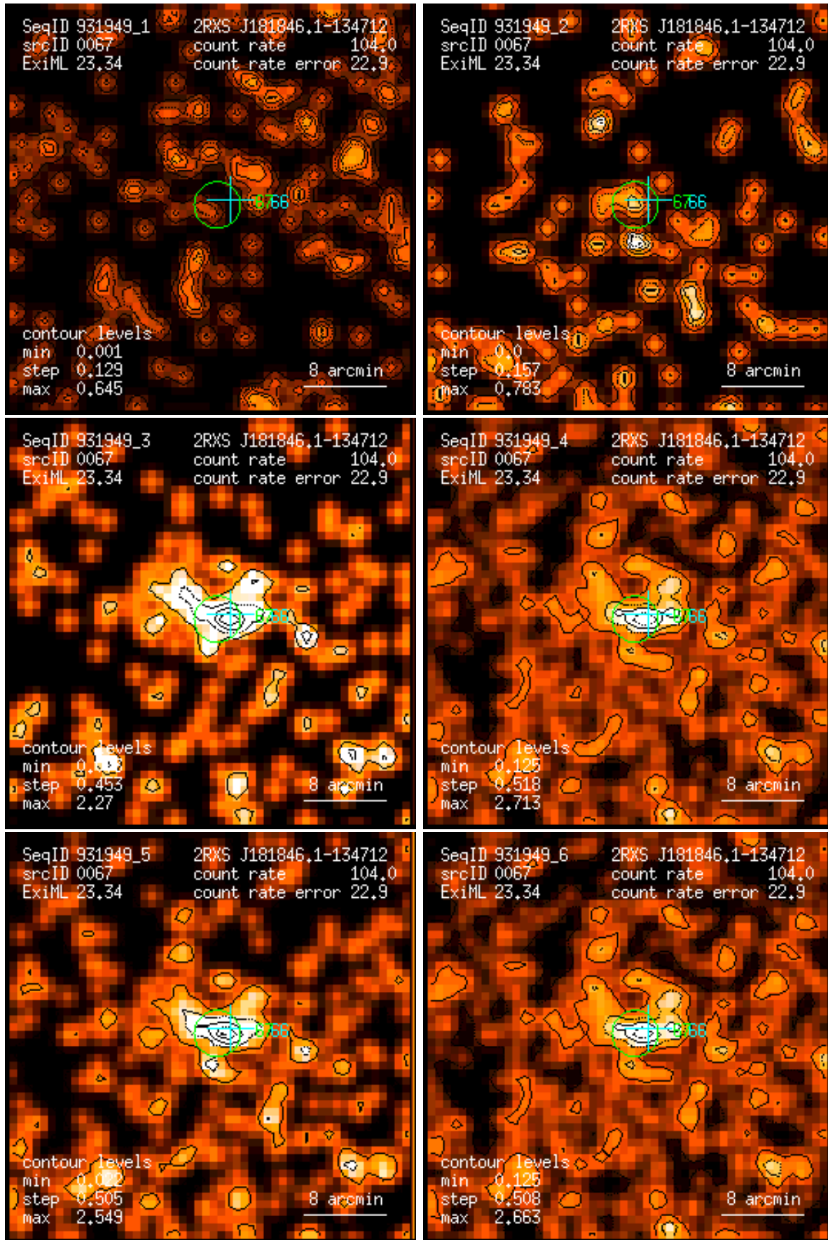
Figure 67: RASS 931949: detection 0067: band rate images, Gaussian filter: (1) PSPC channels 11 – 41, (2) 52 – 90, (3) 91 – 201, (4) 11 – 235, (5) 52 – 201, (6) 11 – 201. Broad band rates in counts/ks. Band rate contour levels in counts/ks/arcmin 2 .
