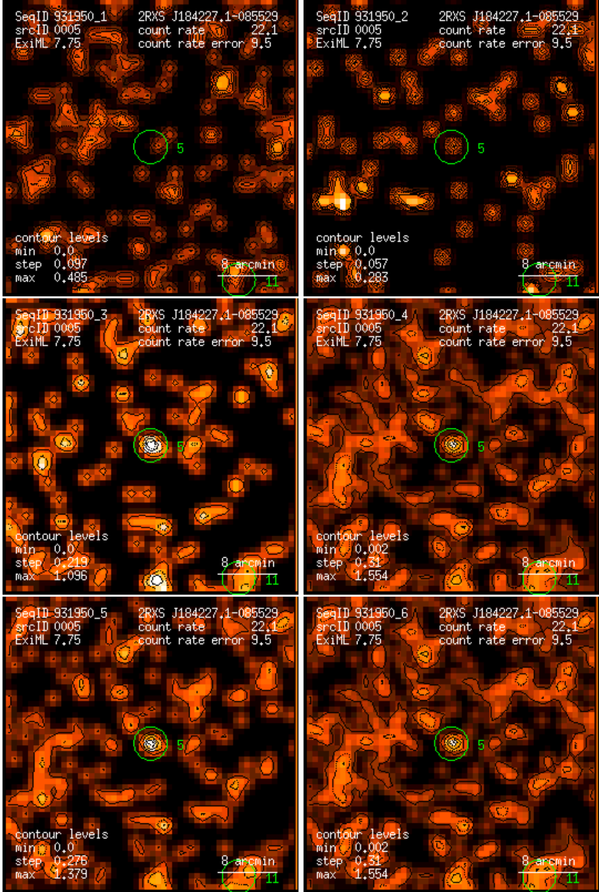
Figure 5: RASS 931950: detection 0005: band rate images, Gaussian filter: (1) PSPC channels 11 – 41, (2) 52 – 90, (3) 91 – 201, (4) 11 – 235, (5) 52 – 201, (6) 11 – 201. Broad band rates in counts/ks. Band rate contour levels in counts/ks/arcmin 2 .
