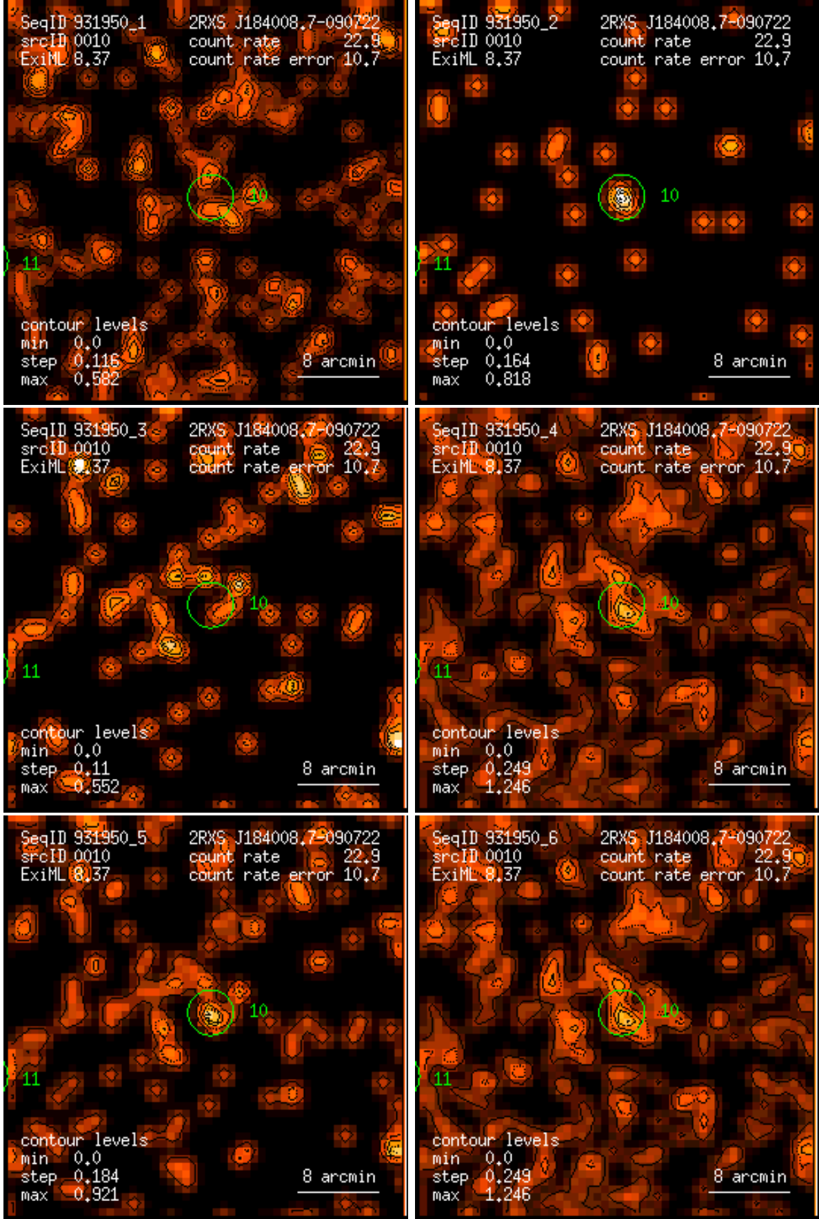
Figure 10: RASS 931950: detection 0010: band rate images, Gaussian filter: (1) PSPC channels 11 – 41, (2) 52 – 90, (3) 91 – 201, (4) 11 – 235, (5) 52 – 201, (6) 11 – 201. Broad band rates in counts/ks. Band rate contour levels in counts/ks/arcmin 2 .
