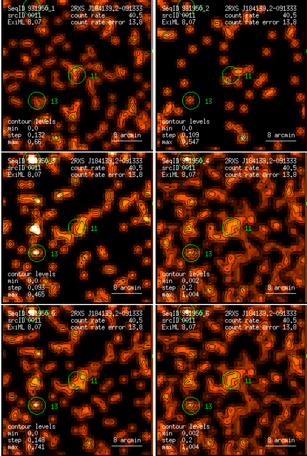
Figure 11: RASS 931950: detection 0011: band rate images, Gaussian filter: (1) PSPC channels 11 – 41, (2) 52 – 90, (3) 91 – 201, (4) 11 – 235, (5) 52 – 201, (6) 11 – 201. Broad band rates in counts/ks. Band rate contour levels in counts/ks/arcmin 2 .
