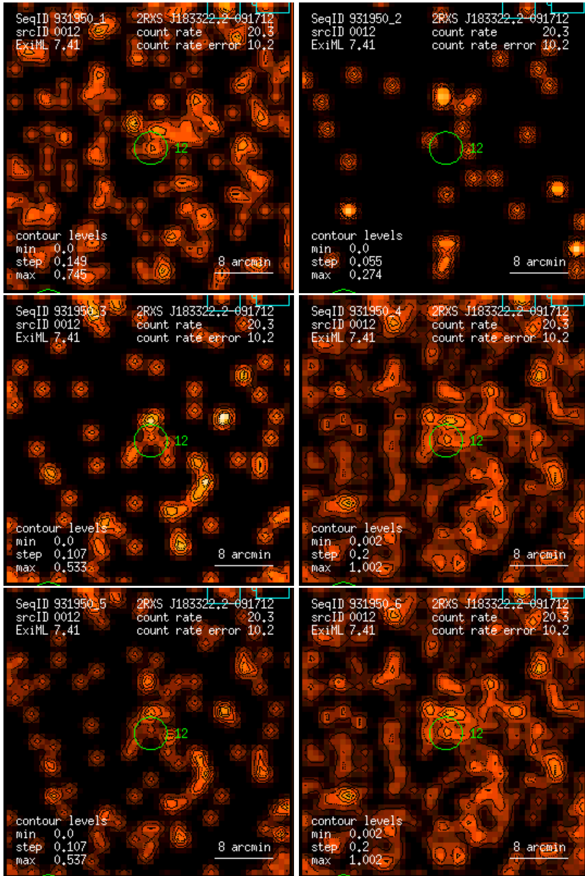
Figure 12: RASS 931950: detection 0012: band rate images, Gaussian filter: (1) PSPC channels 11 – 41, (2) 52 – 90, (3) 91 – 201, (4) 11 – 235, (5) 52 – 201, (6) 11 – 201. Broad band rates in counts/ks. Band rate contour levels in counts/ks/arcmin 2 .
