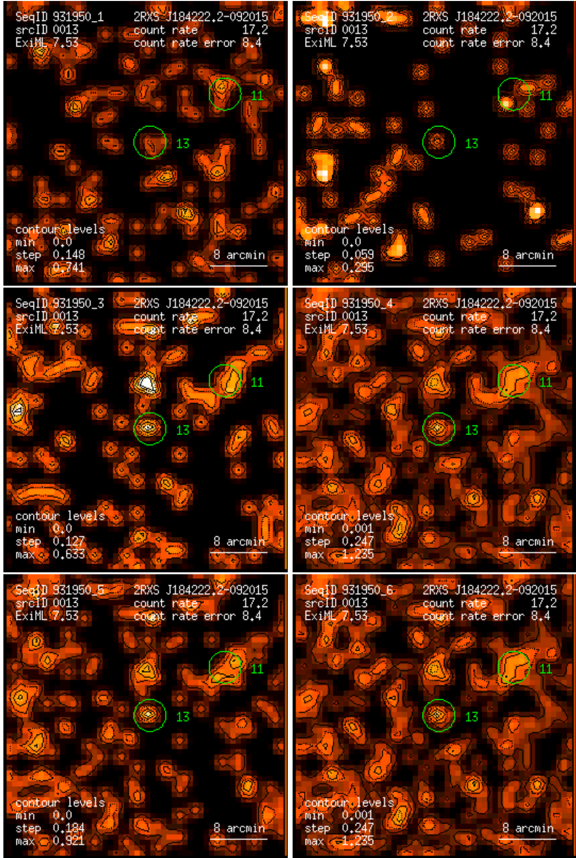
Figure 13: RASS 931950: detection 0013: band rate images, Gaussian filter: (1) PSPC channels 11 – 41, (2) 52 – 90, (3) 91 – 201, (4) 11 – 235, (5) 52 – 201, (6) 11 – 201. Broad band rates in counts/ks. Band rate contour levels in counts/ks/arcmin 2 .
