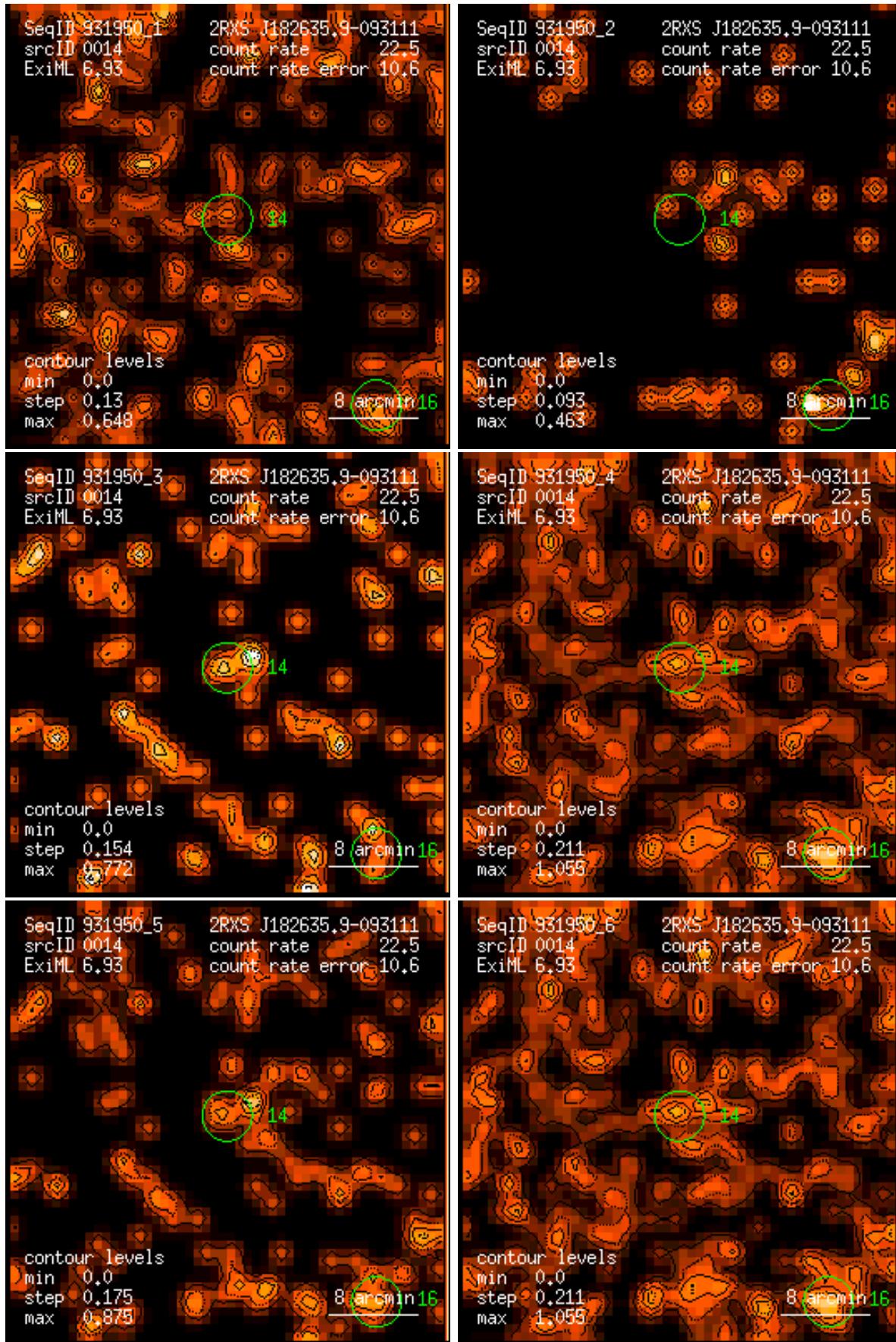
Figure 14: RASS 931950: detection 0014: band rate images, Gaussian filter: (1) PSPC channels 11 – 41, (2) 52 – 90, (3) 91 – 201, (4) 11 – 235, (5) 52 – 201, (6) 11 – 201. Broad band rates in counts/ks. Band rate contour levels in counts/ks/arcmin 2 .
