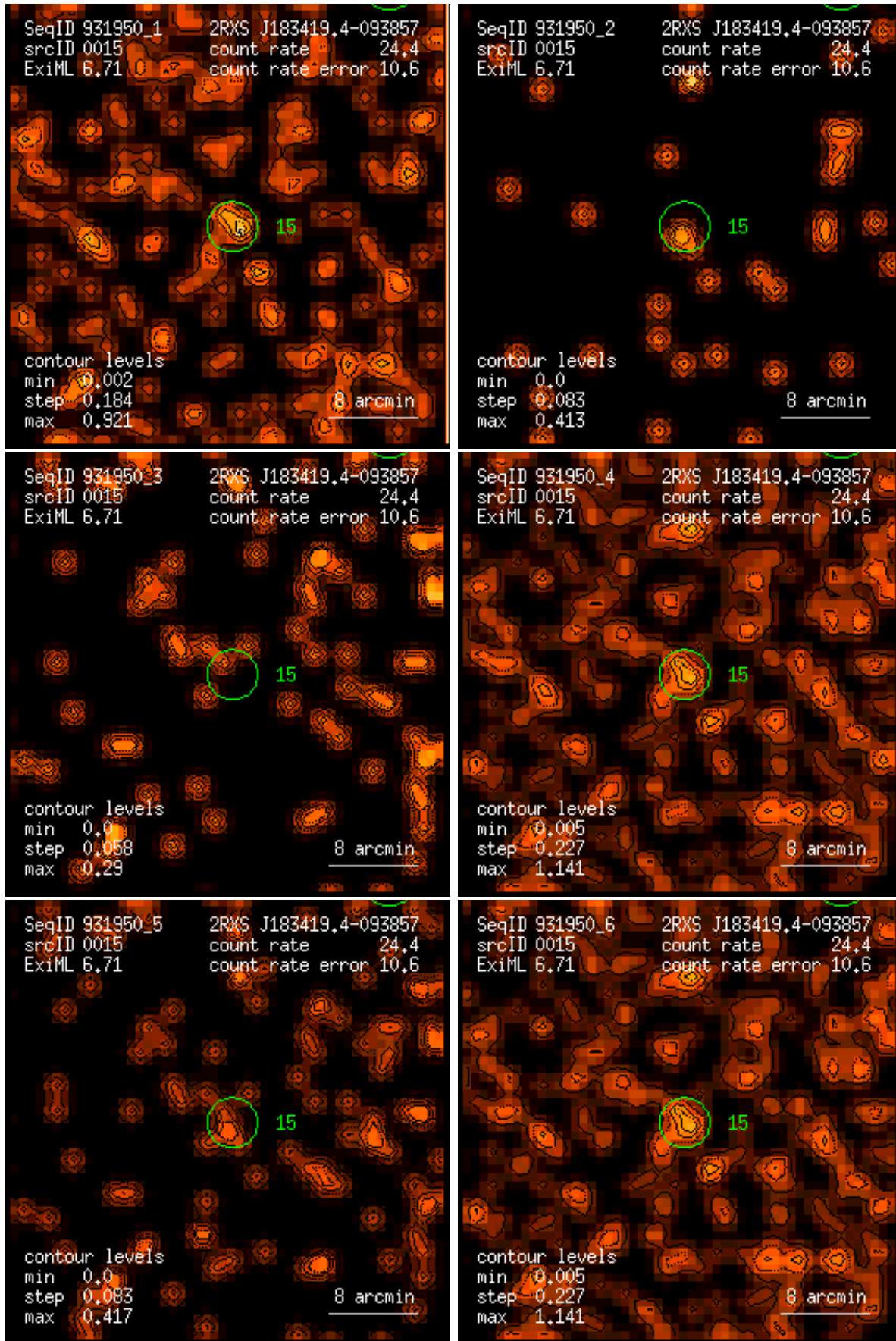
Figure 15: RASS 931950: detection 0015: band rate images, Gaussian filter: (1) PSPC channels 11 – 41, (2) 52 – 90, (3) 91 – 201, (4) 11 – 235, (5) 52 – 201, (6) 11 – 201. Broad band rates in counts/ks. Band rate contour levels in counts/ks/arcmin 2 .
