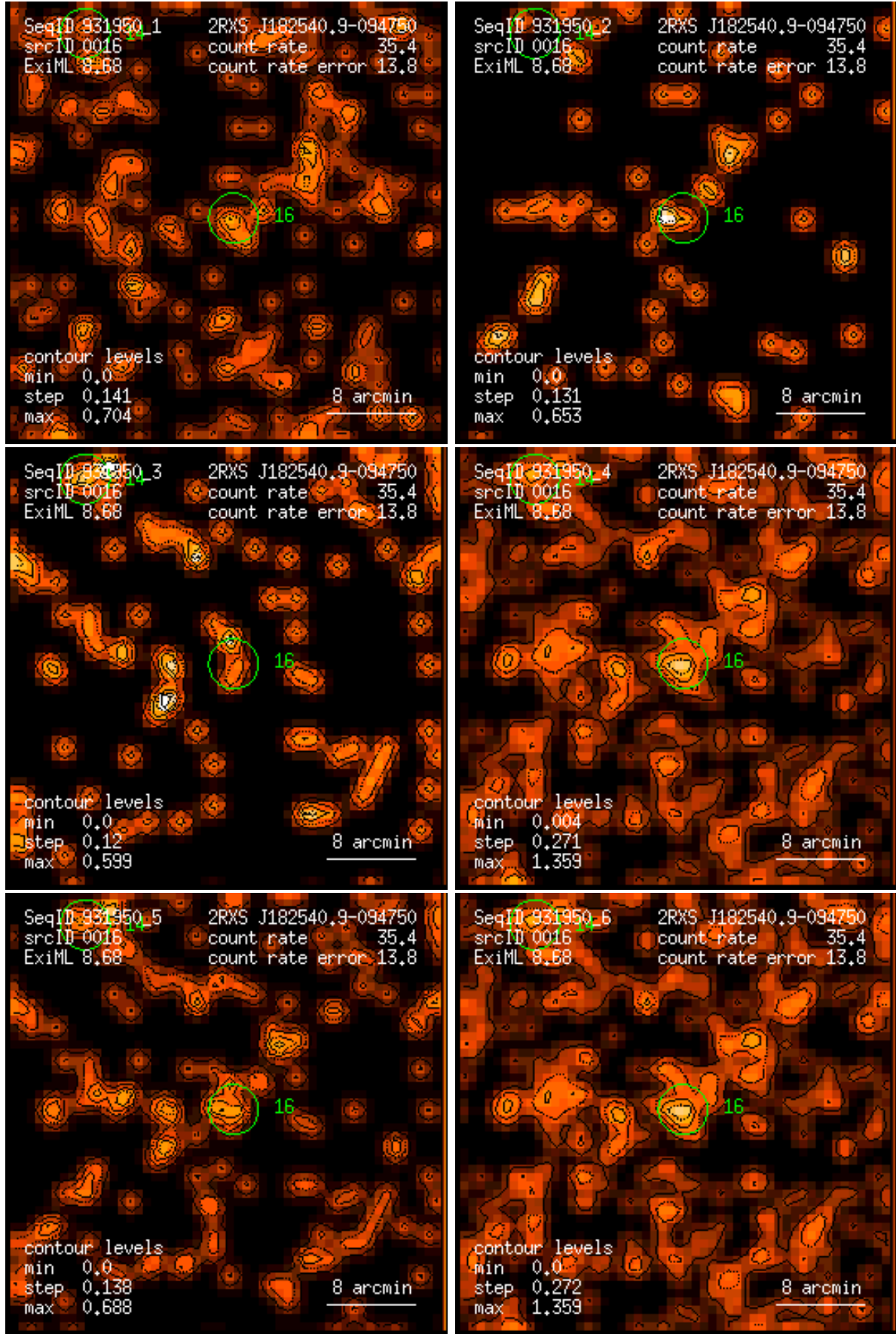
Figure 16: RASS 931950: detection 0016: band rate images, Gaussian filter: (1) PSPC channels 11 – 41, (2) 52 – 90, (3) 91 – 201, (4) 11 – 235, (5) 52 – 201, (6) 11 – 201. Broad band rates in counts/ks. Band rate contour levels in counts/ks/arcmin 2 .
