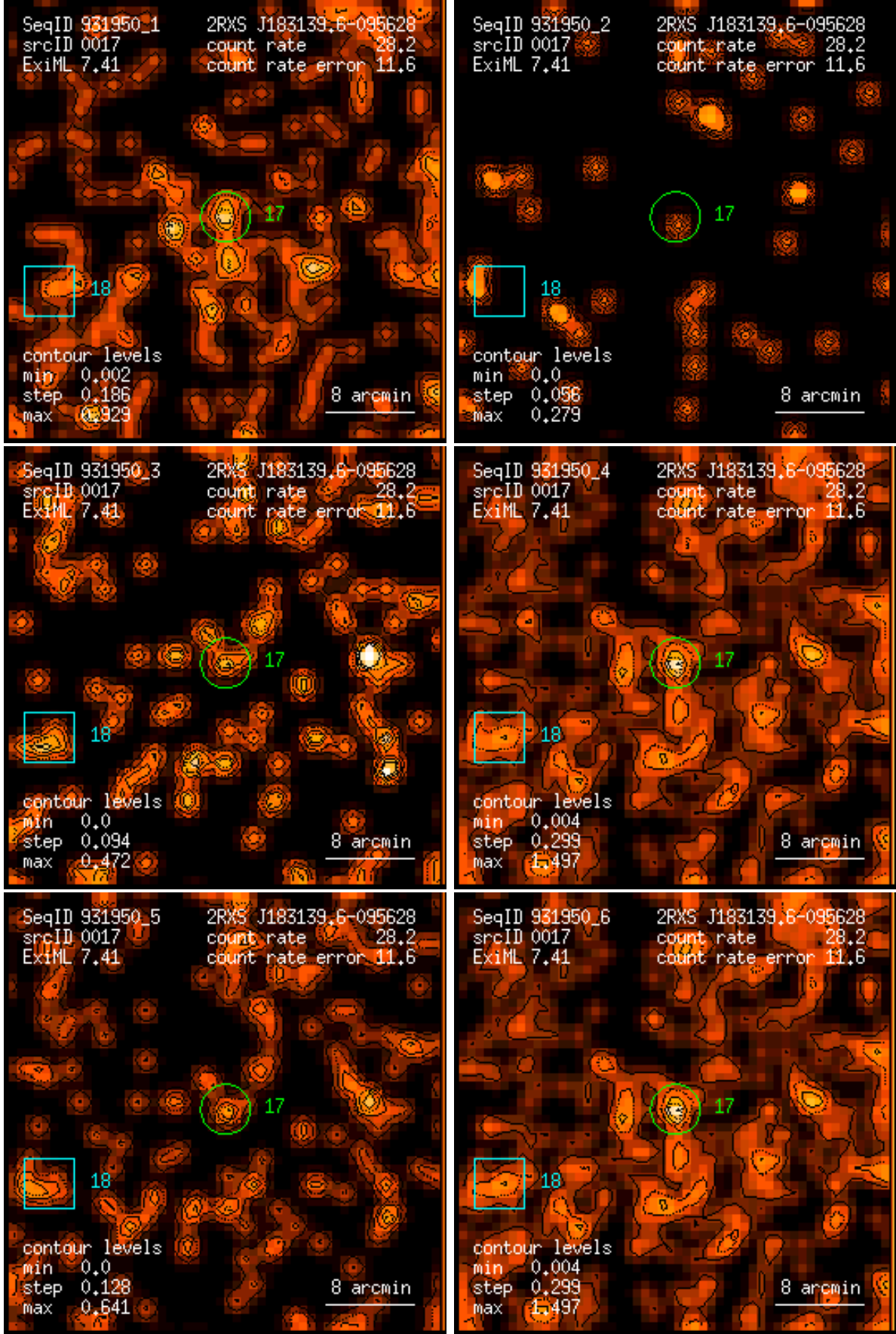
Figure 17: RASS 931950: detection 0017: band rate images, Gaussian filter: (1) PSPC channels 11 – 41, (2) 52 – 90, (3) 91 – 201, (4) 11 – 235, (5) 52 – 201, (6) 11 – 201. Broad band rates in counts/ks. Band rate contour levels in counts/ks/arcmin 2 .
