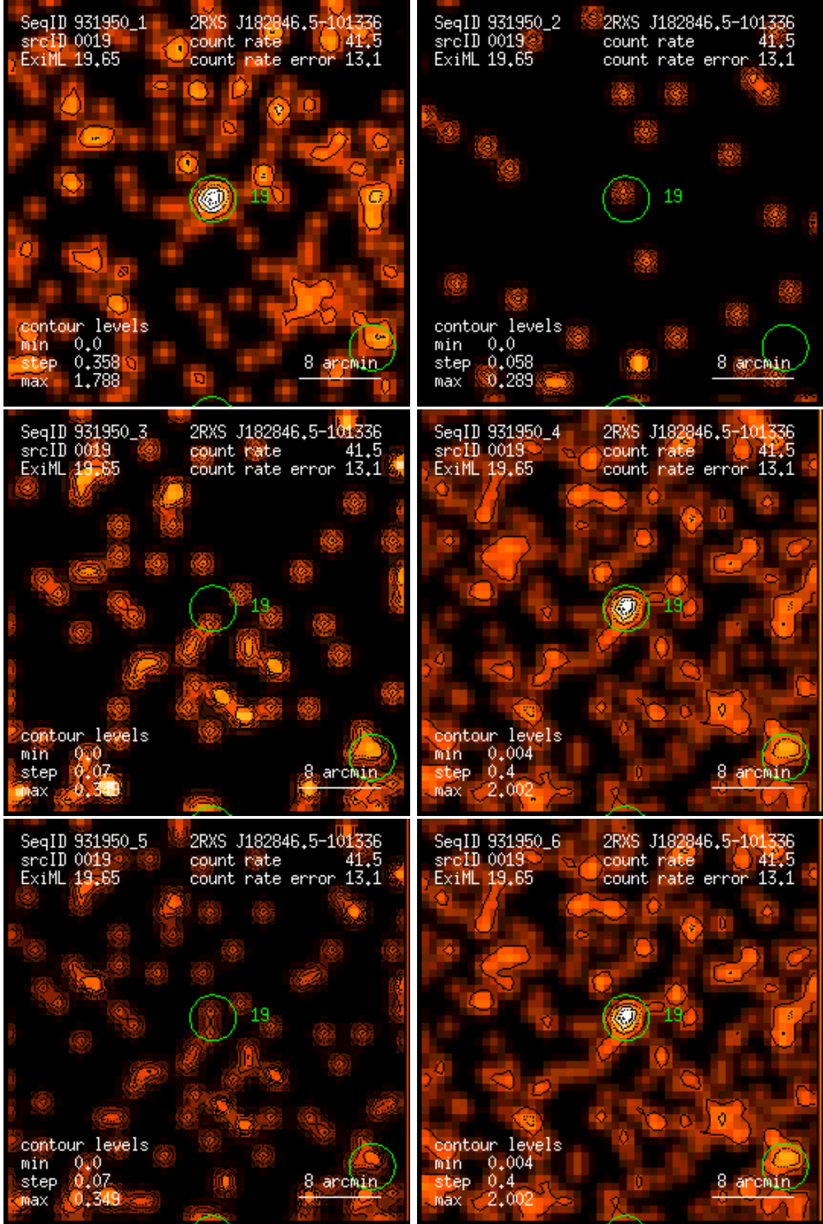
Figure 19: RASS 931950: detection 0019: band rate images, Gaussian filter: (1) PSPC channels 11 – 41, (2) 52 – 90, (3) 91 – 201, (4) 11 – 235, (5) 52 – 201, (6) 11 – 201. Broad band rates in counts/ks. Band rate contour levels in counts/ks/arcmin 2 .
