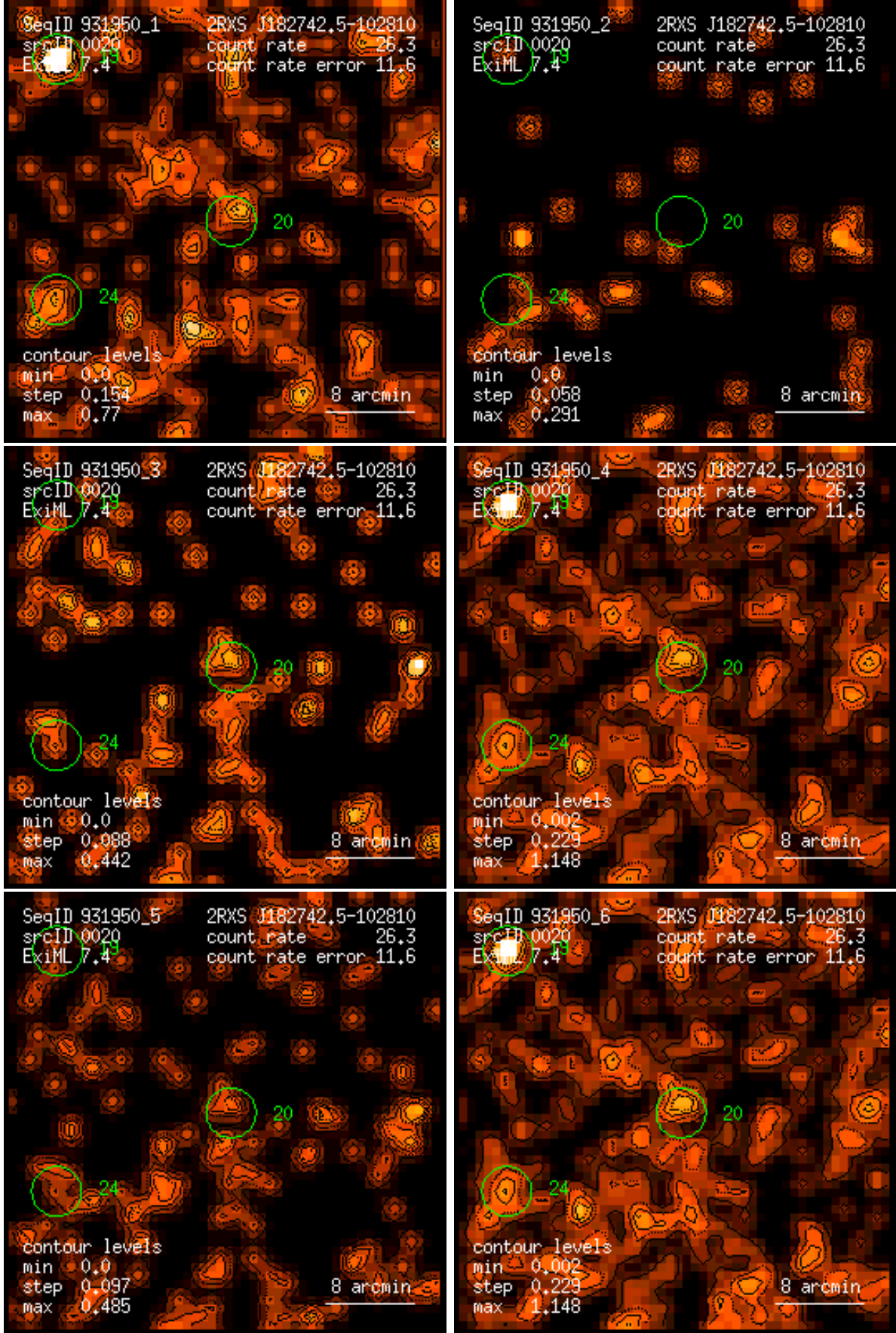
Figure 20: RASS 931950: detection 0020: band rate images, Gaussian filter: (1) PSPC channels 11 – 41, (2) 52 – 90, (3) 91 – 201, (4) 11 – 235, (5) 52 – 201, (6) 11 – 201. Broad band rates in counts/ks. Band rate contour levels in counts/ks/arcmin 2 .
