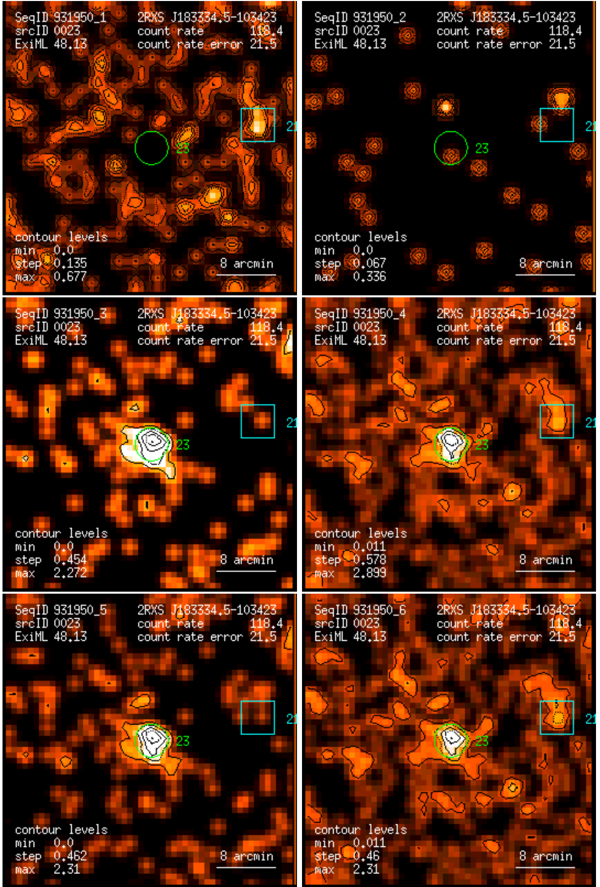
Figure 23: RASS 931950: detection 0023: band rate images, Gaussian filter: (1) PSPC channels 11 – 41, (2) 52 – 90, (3) 91 – 201, (4) 11 – 235, (5) 52 – 201, (6) 11 – 201. Broad band rates in counts/ks. Band rate contour levels in counts/ks/arcmin 2 .
