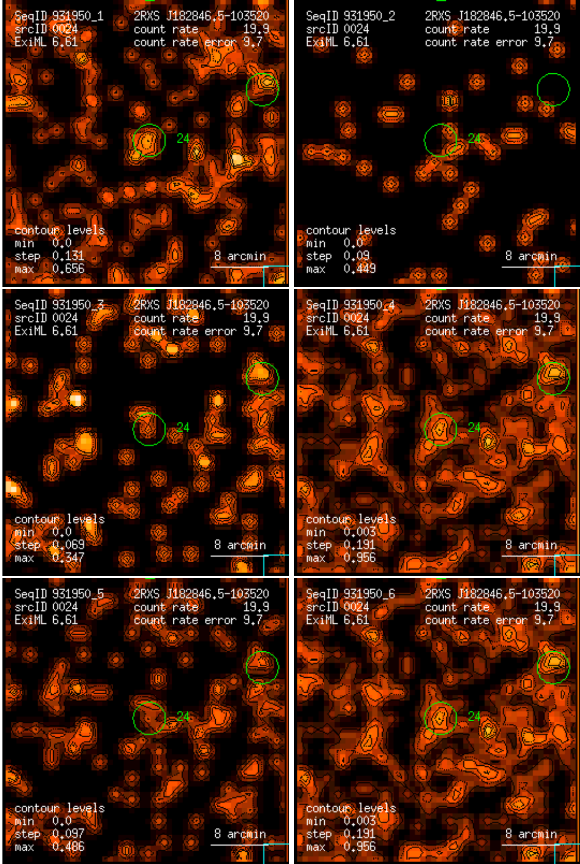
Figure 24: RASS 931950: detection 0024: band rate images, Gaussian filter: (1) PSPC channels 11 – 41, (2) 52 – 90, (3) 91 – 201, (4) 11 – 235, (5) 52 – 201, (6) 11 – 201. Broad band rates in counts/ks. Band rate contour levels in counts/ks/arcmin 2 .
