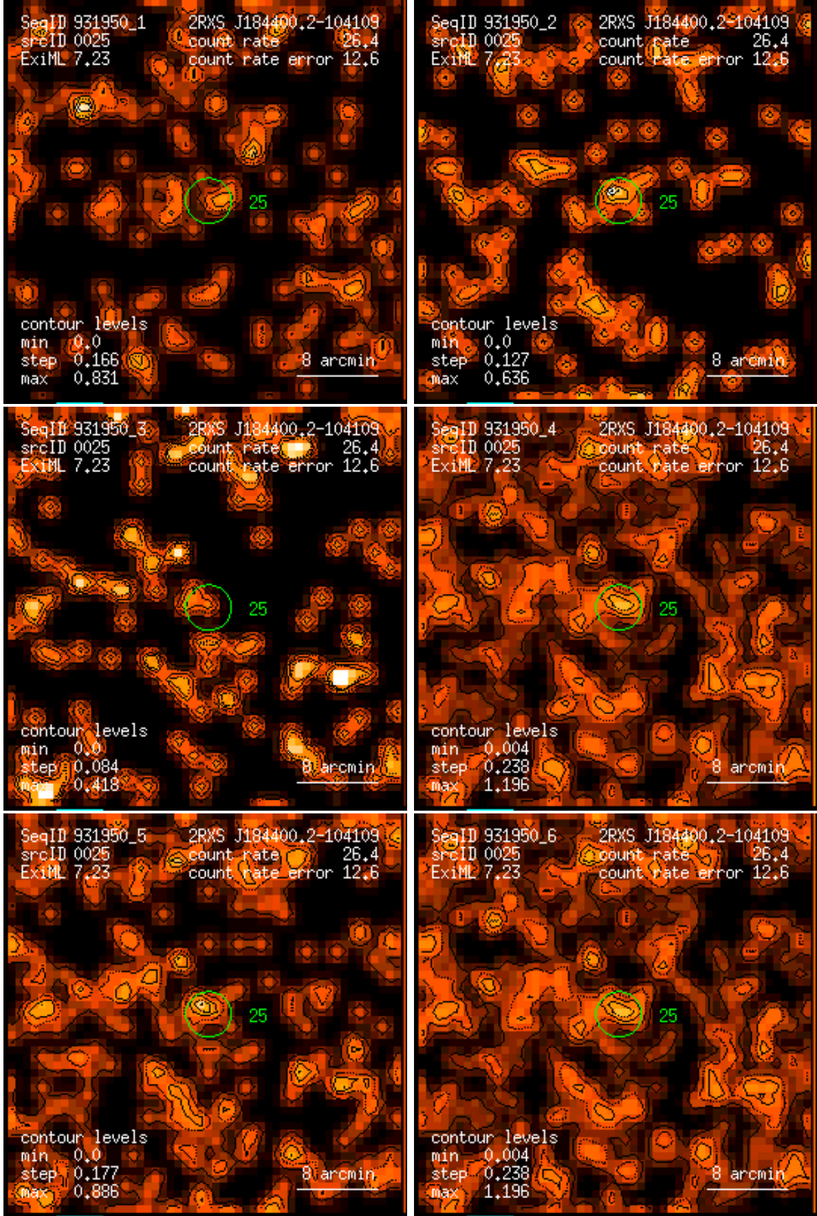
Figure 25: RASS 931950: detection 0025: band rate images, Gaussian filter: (1) PSPC channels 11 – 41, (2) 52 – 90, (3) 91 – 201, (4) 11 – 235, (5) 52 – 201, (6) 11 – 201. Broad band rates in counts/ks. Band rate contour levels in counts/ks/arcmin 2 .
