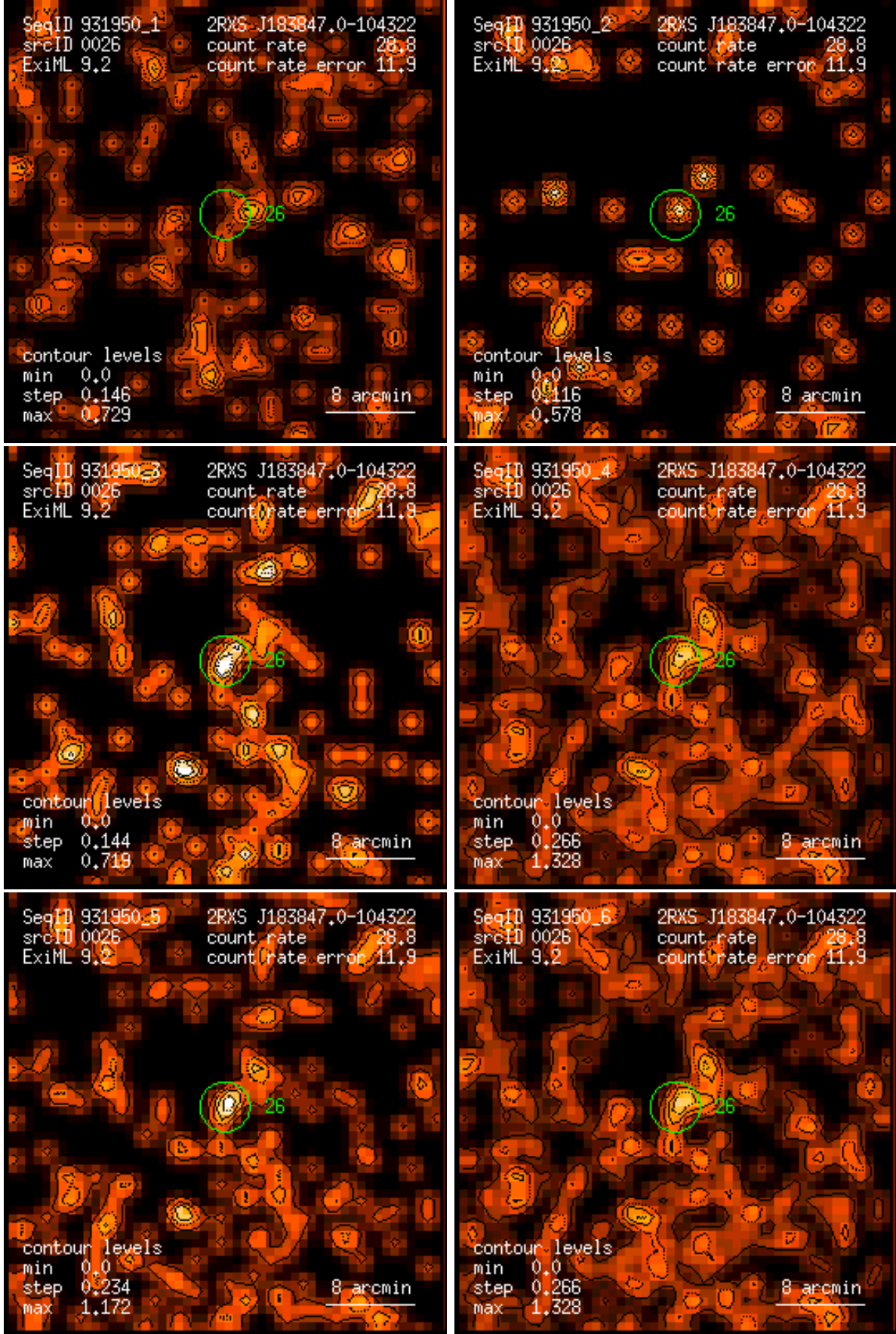
Figure 26: RASS 931950: detection 0026: band rate images, Gaussian filter: (1) PSPC channels 11 – 41, (2) 52 – 90, (3) 91 – 201, (4) 11 – 235, (5) 52 – 201, (6) 11 – 201. Broad band rates in counts/ks. Band rate contour levels in counts/ks/arcmin 2 .
