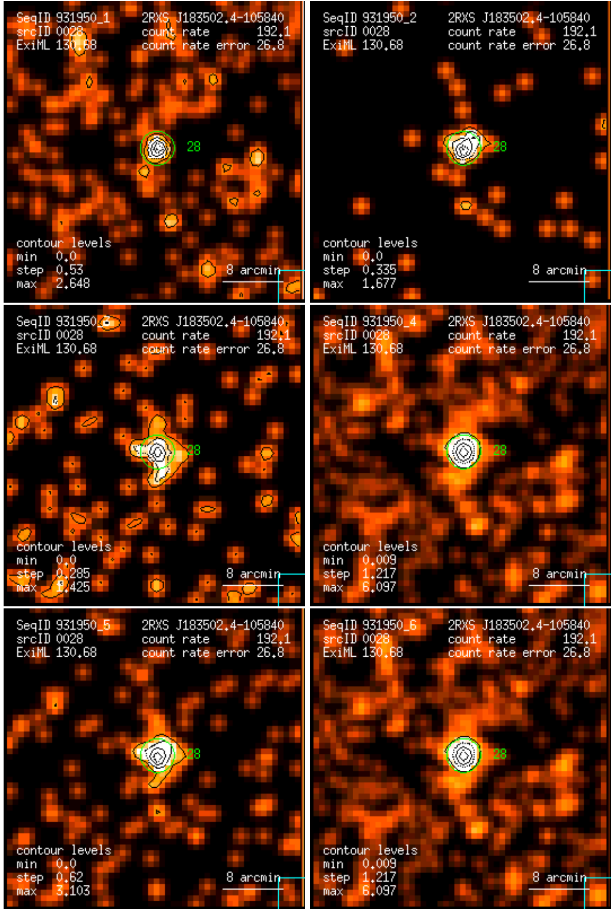
Figure 28: RASS 931950: detection 0028: band rate images, Gaussian filter: (1) PSPC channels 11 – 41, (2) 52 – 90, (3) 91 – 201, (4) 11 – 235, (5) 52 – 201, (6) 11 – 201. Broad band rates in counts/ks. Band rate contour levels in counts/ks/arcmin 2 .
