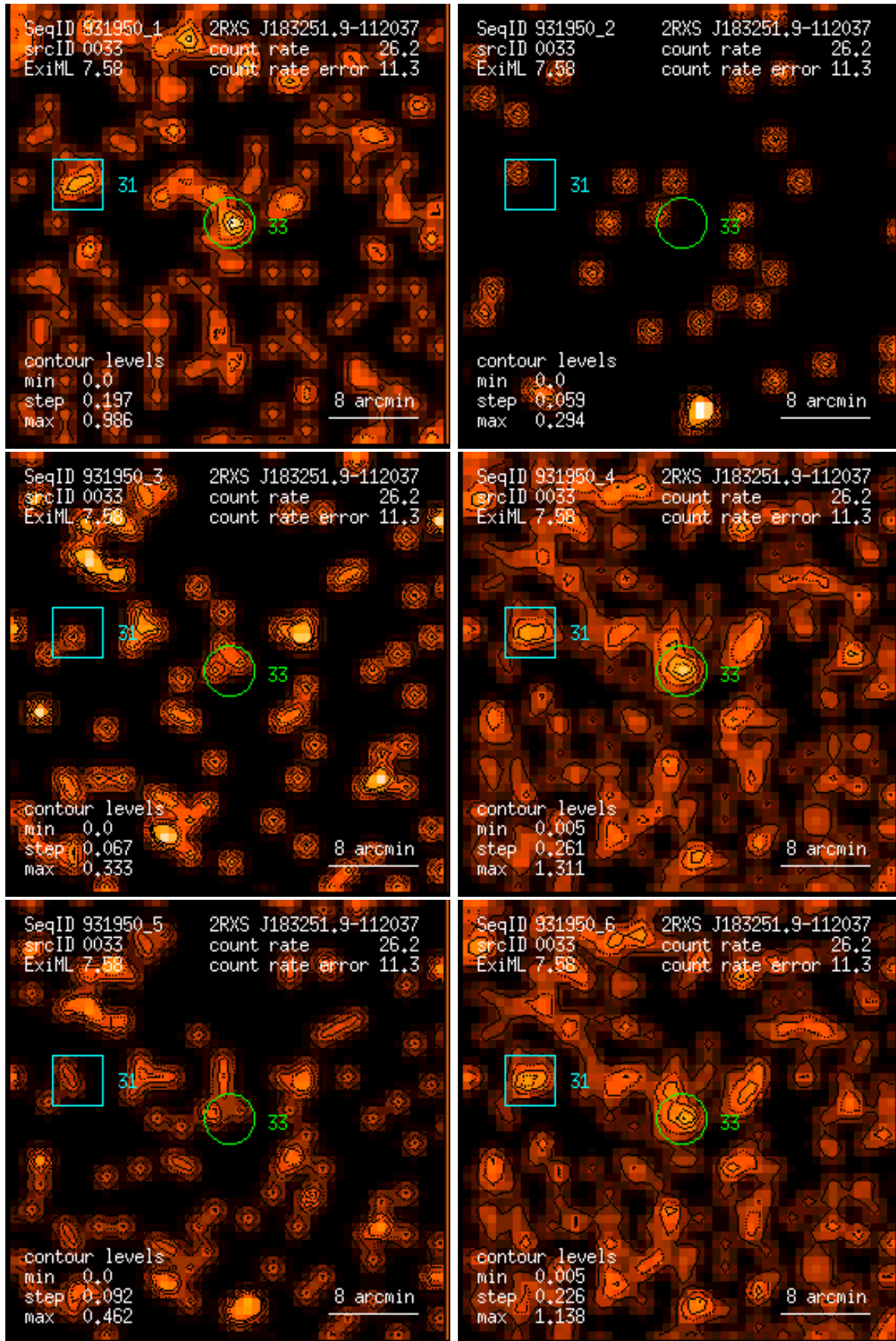
Figure 33: RASS 931950: detection 0033: band rate images, Gaussian filter: (1) PSPC channels 11 – 41, (2) 52 – 90, (3) 91 – 201, (4) 11 – 235, (5) 52 – 201, (6) 11 – 201. Broad band rates in counts/ks. Band rate contour levels in counts/ks/arcmin 2 .
