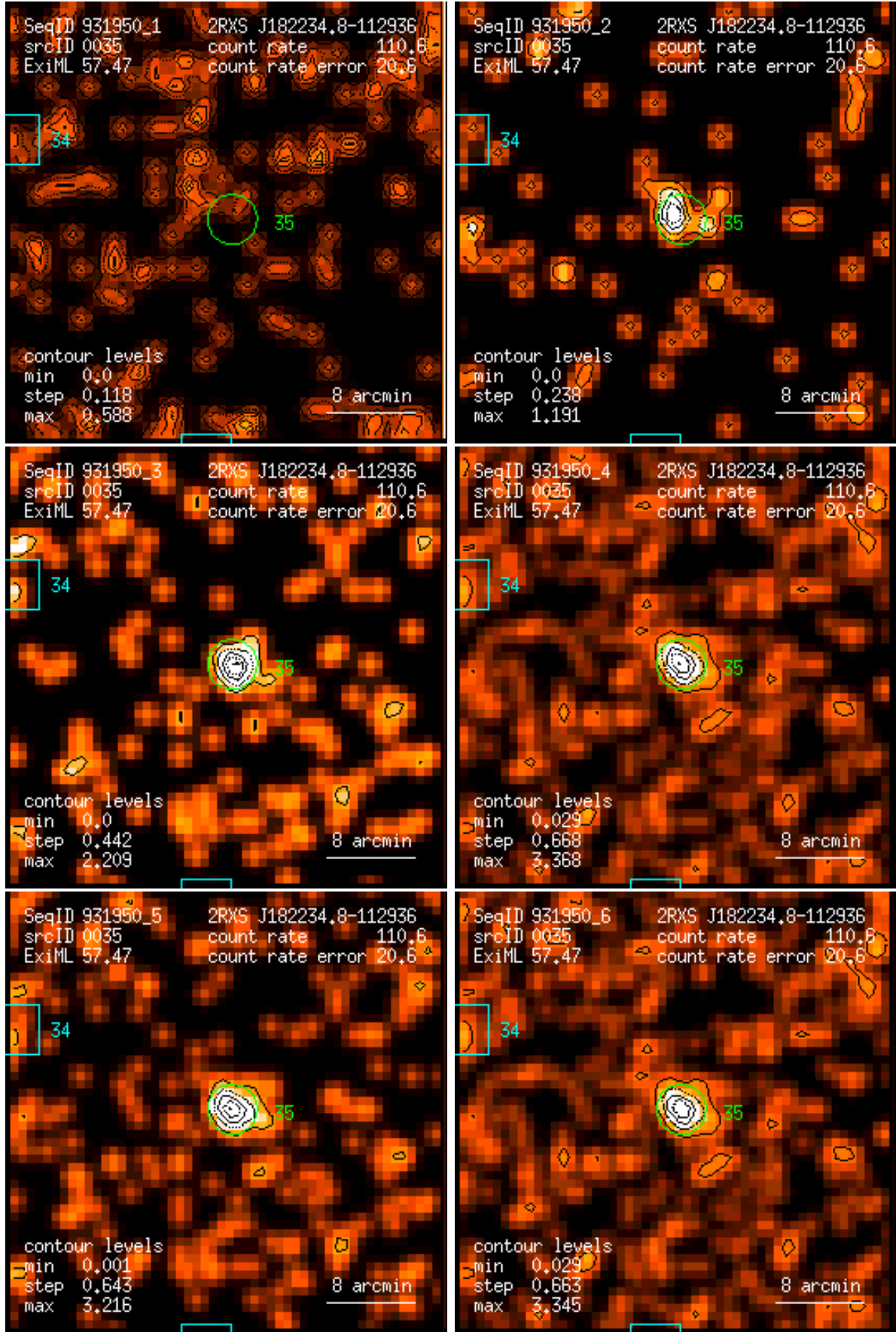
Figure 35: RASS 931950: detection 0035: band rate images, Gaussian filter: (1) PSPC channels 11 – 41, (2) 52 – 90, (3) 91 – 201, (4) 11 – 235, (5) 52 – 201, (6) 11 – 201. Broad band rates in counts/ks. Band rate contour levels in counts/ks/arcmin 2 .
