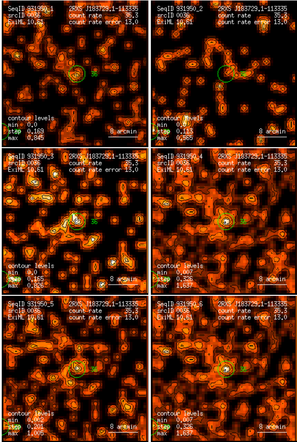
Figure 36: RASS 931950: detection 0036: band rate images, Gaussian filter: (1) PSPC channels 11 – 41, (2) 52 – 90, (3) 91 – 201, (4) 11 – 235, (5) 52 – 201, (6) 11 – 201. Broad band rates in counts/ks. Band rate contour levels in counts/ks/arcmin 2 .
