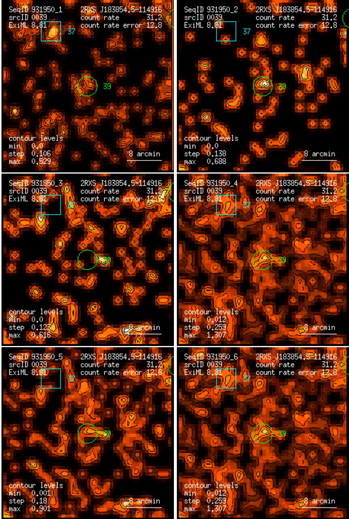
Figure 39: RASS 931950: detection 0039: band rate images, Gaussian filter: (1) PSPC channels 11 – 41, (2) 52 – 90, (3) 91 – 201, (4) 11 – 235, (5) 52 – 201, (6) 11 – 201. Broad band rates in counts/ks. Band rate contour levels in counts/ks/arcmin 2 .
