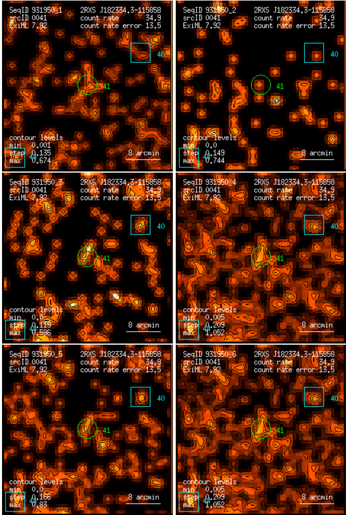
Figure 41: RASS 931950: detection 0041: band rate images, Gaussian filter: (1) PSPC channels 11 – 41, (2) 52 – 90, (3) 91 – 201, (4) 11 – 235, (5) 52 – 201, (6) 11 – 201. Broad band rates in counts/ks. Band rate contour levels in counts/ks/arcmin 2 .
