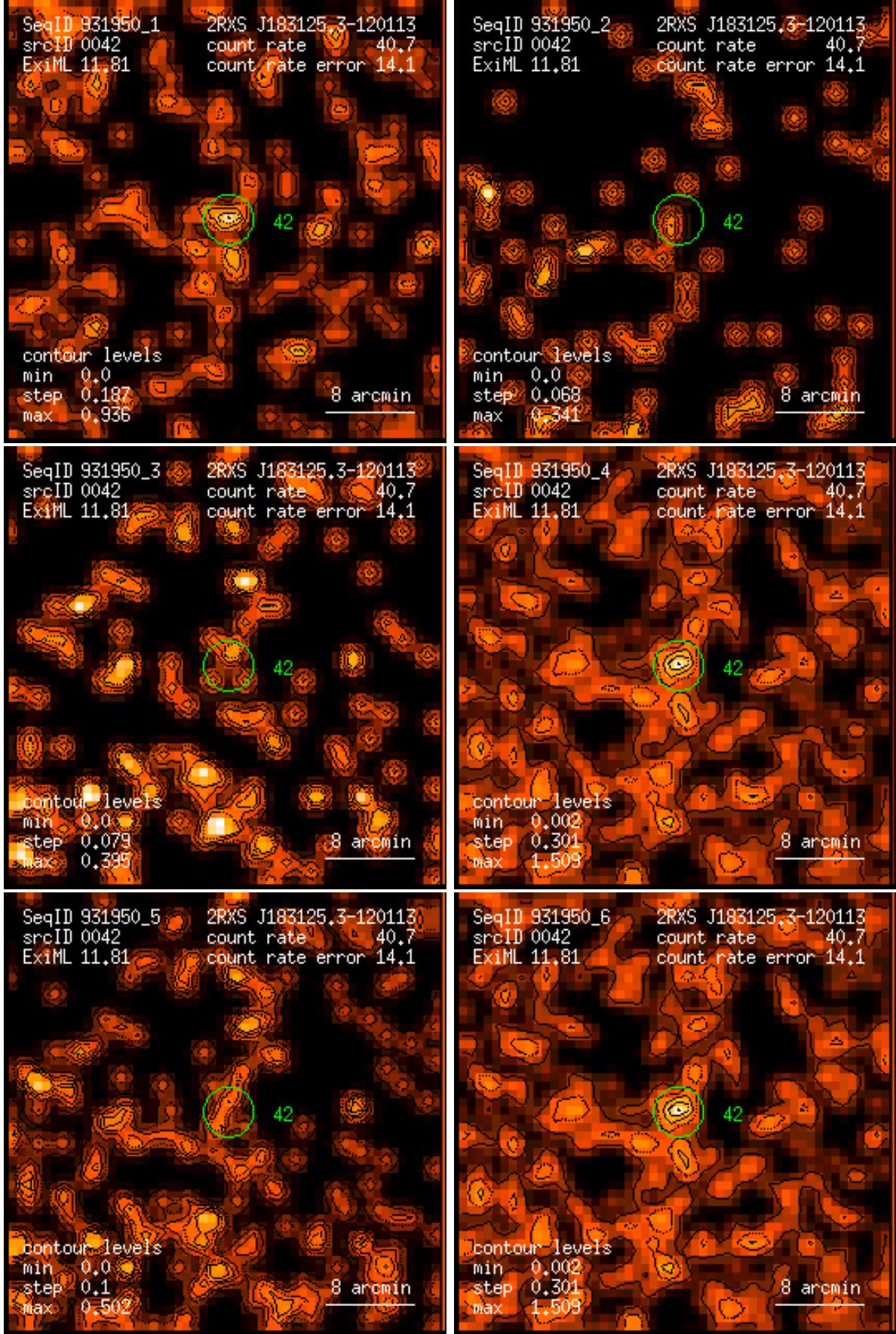
Figure 42: RASS 931950: detection 0042: band rate images, Gaussian filter: (1) PSPC channels 11 – 41, (2) 52 – 90, (3) 91 – 201, (4) 11 – 235, (5) 52 – 201, (6) 11 – 201. Broad band rates in counts/ks. Band rate contour levels in counts/ks/arcmin 2 .
