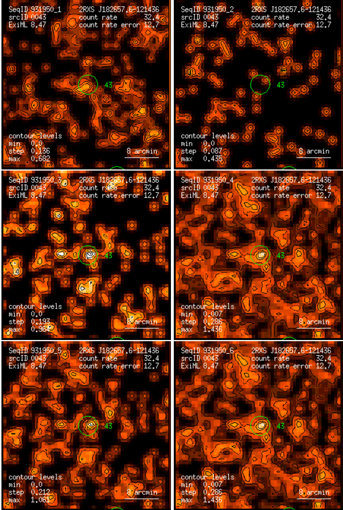
Figure 43: RASS 931950: detection 0043: band rate images, Gaussian filter: (1) PSPC channels 11 – 41, (2) 52 – 90, (3) 91 – 201, (4) 11 – 235, (5) 52 – 201, (6) 11 – 201. Broad band rates in counts/ks. Band rate contour levels in counts/ks/arcmin 2 .
