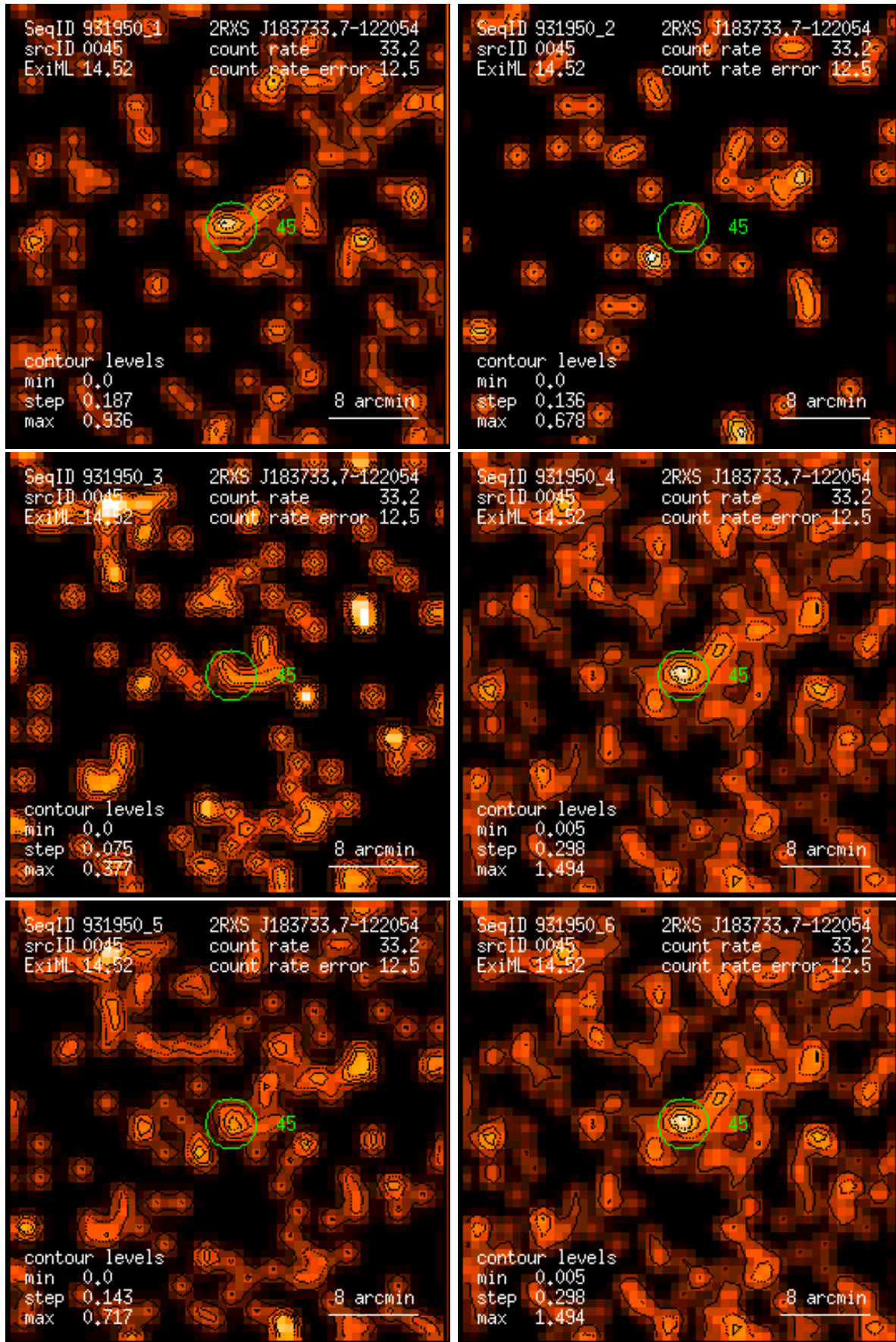
Figure 45: RASS 931950: detection 0045: band rate images, Gaussian filter: (1) PSPC channels 11 – 41, (2) 52 – 90, (3) 91 – 201, (4) 11 – 235, (5) 52 – 201, (6) 11 – 201. Broad band rates in counts/ks. Band rate contour levels in counts/ks/arcmin 2 .
