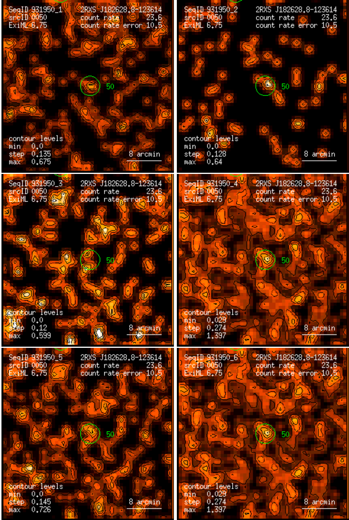
Figure 50: RASS 931950: detection 0050: band rate images, Gaussian filter: (1) PSPC channels 11 – 41, (2) 52 – 90, (3) 91 – 201, (4) 11 – 235, (5) 52 – 201, (6) 11 – 201. Broad band rates in counts/ks. Band rate contour levels in counts/ks/arcmin 2 .
