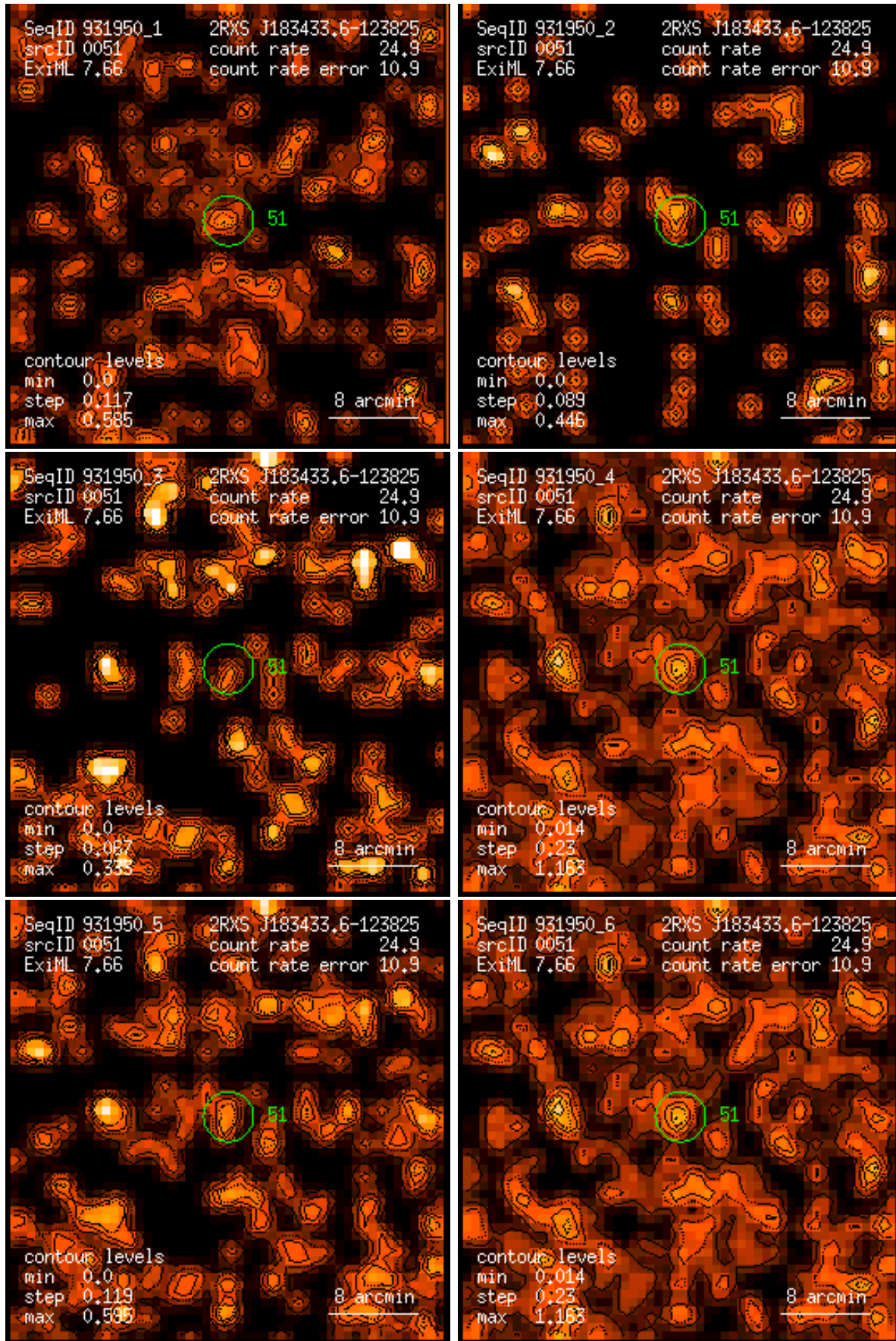
Figure 51: RASS 931950: detection 0051: band rate images, Gaussian filter: (1) PSPC channels 11 – 41, (2) 52 – 90, (3) 91 – 201, (4) 11 – 235, (5) 52 – 201, (6) 11 – 201. Broad band rates in counts/ks. Band rate contour levels in counts/ks/arcmin 2 .
