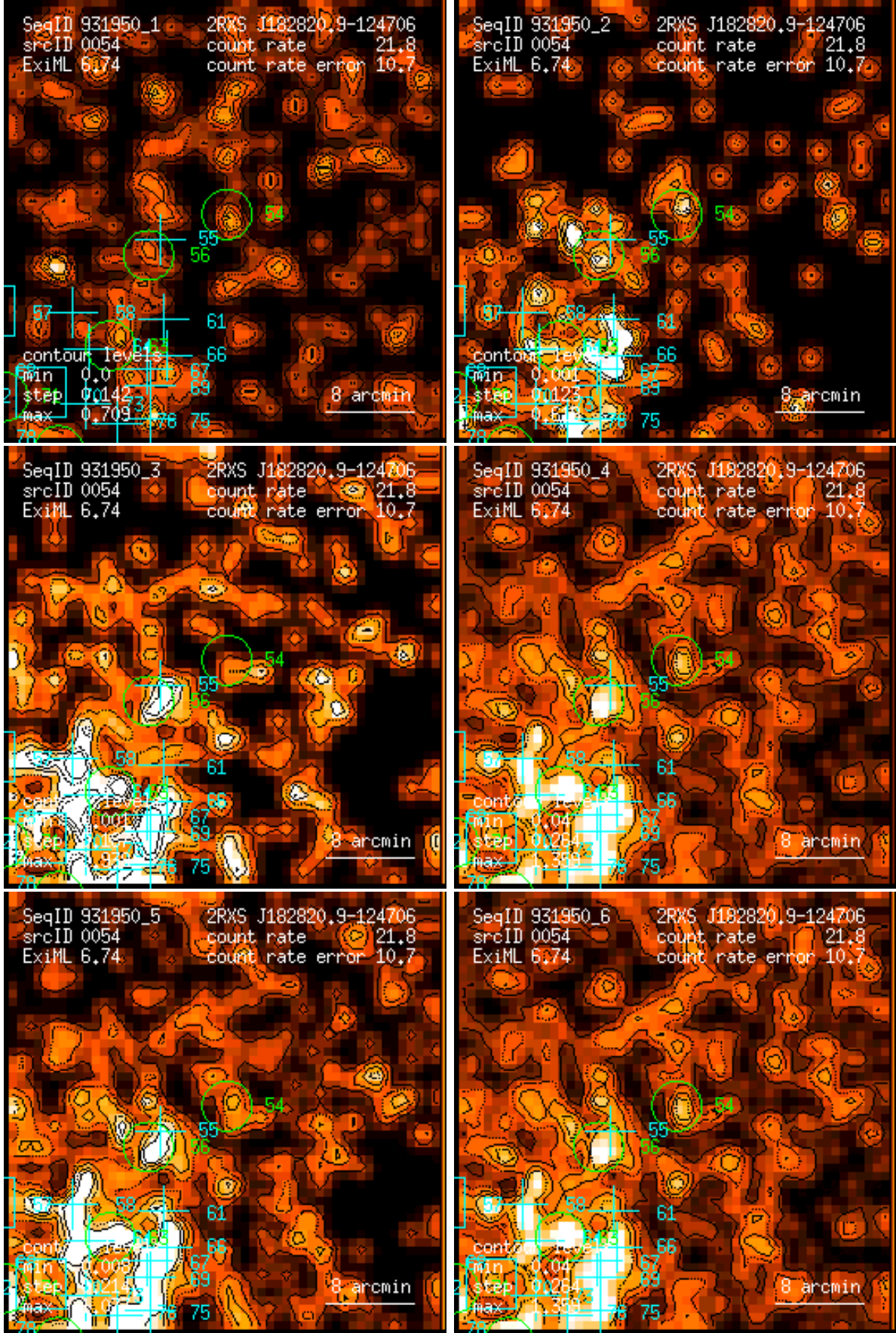
Figure 54: RASS 931950: detection 0054: band rate images, Gaussian filter: (1) PSPC channels 11 – 41, (2) 52 – 90, (3) 91 – 201, (4) 11 – 235, (5) 52 – 201, (6) 11 – 201. Broad band rates in counts/ks. Band rate contour levels in counts/ks/arcmin 2 .
