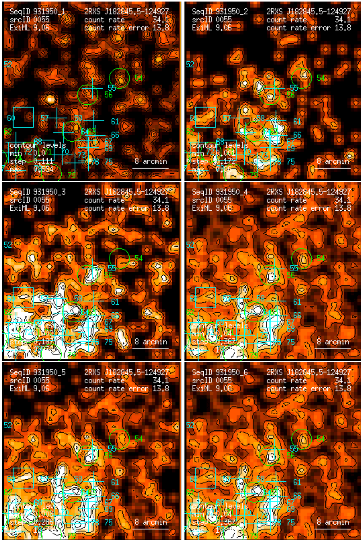
Figure 55: RASS 931950: detection 0055: band rate images, Gaussian filter: (1) PSPC channels 11 – 41, (2) 52 – 90, (3) 91 – 201, (4) 11 – 235, (5) 52 – 201, (6) 11 – 201. Broad band rates in counts/ks. Band rate contour levels in counts/ks/arcmin 2 .
