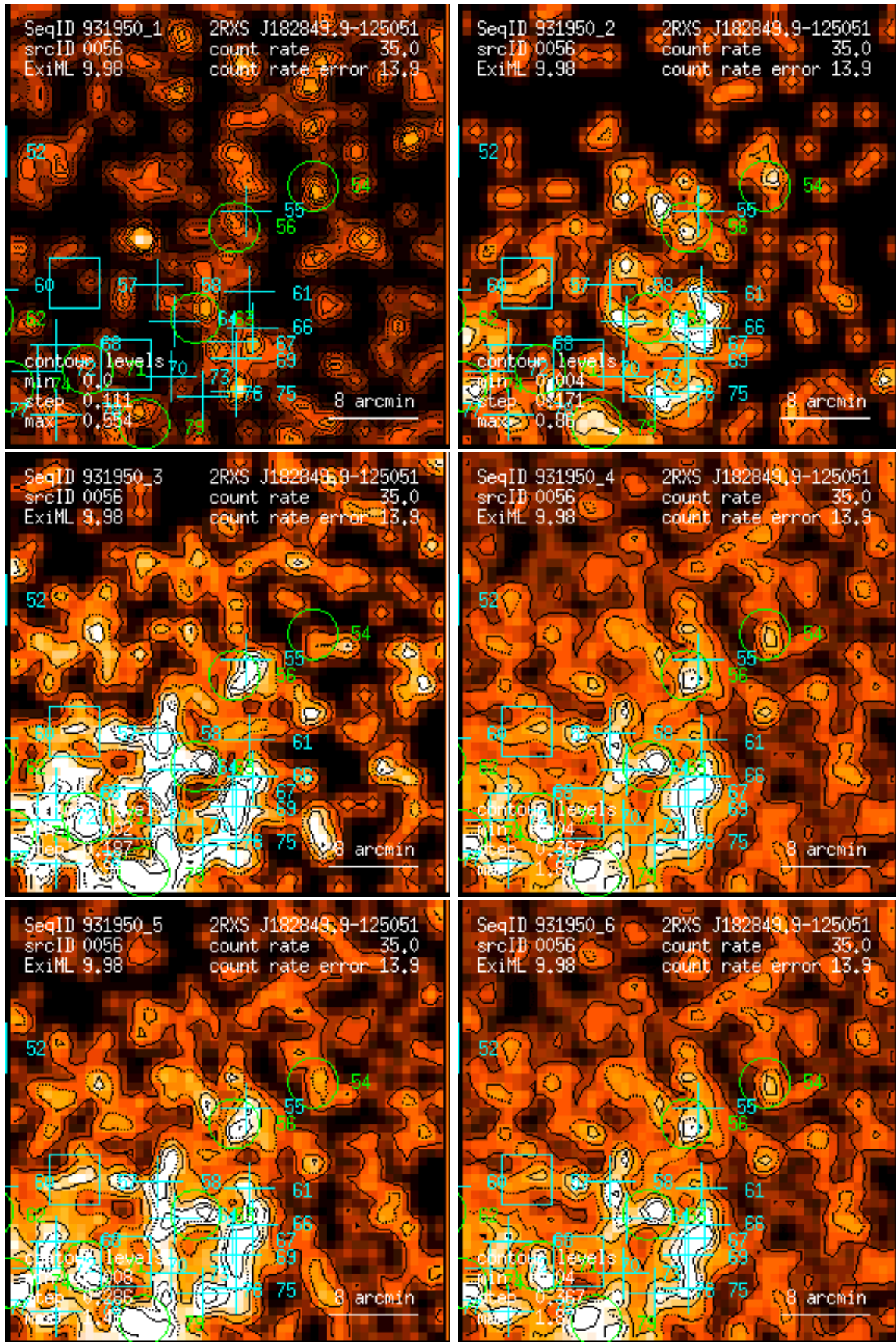
Figure 56: RASS 931950: detection 0056: band rate images, Gaussian filter: (1) PSPC channels 11 – 41, (2) 52 – 90, (3) 91 – 201, (4) 11 – 235, (5) 52 – 201, (6) 11 – 201. Broad band rates in counts/ks. Band rate contour levels in counts/ks/arcmin 2 .
