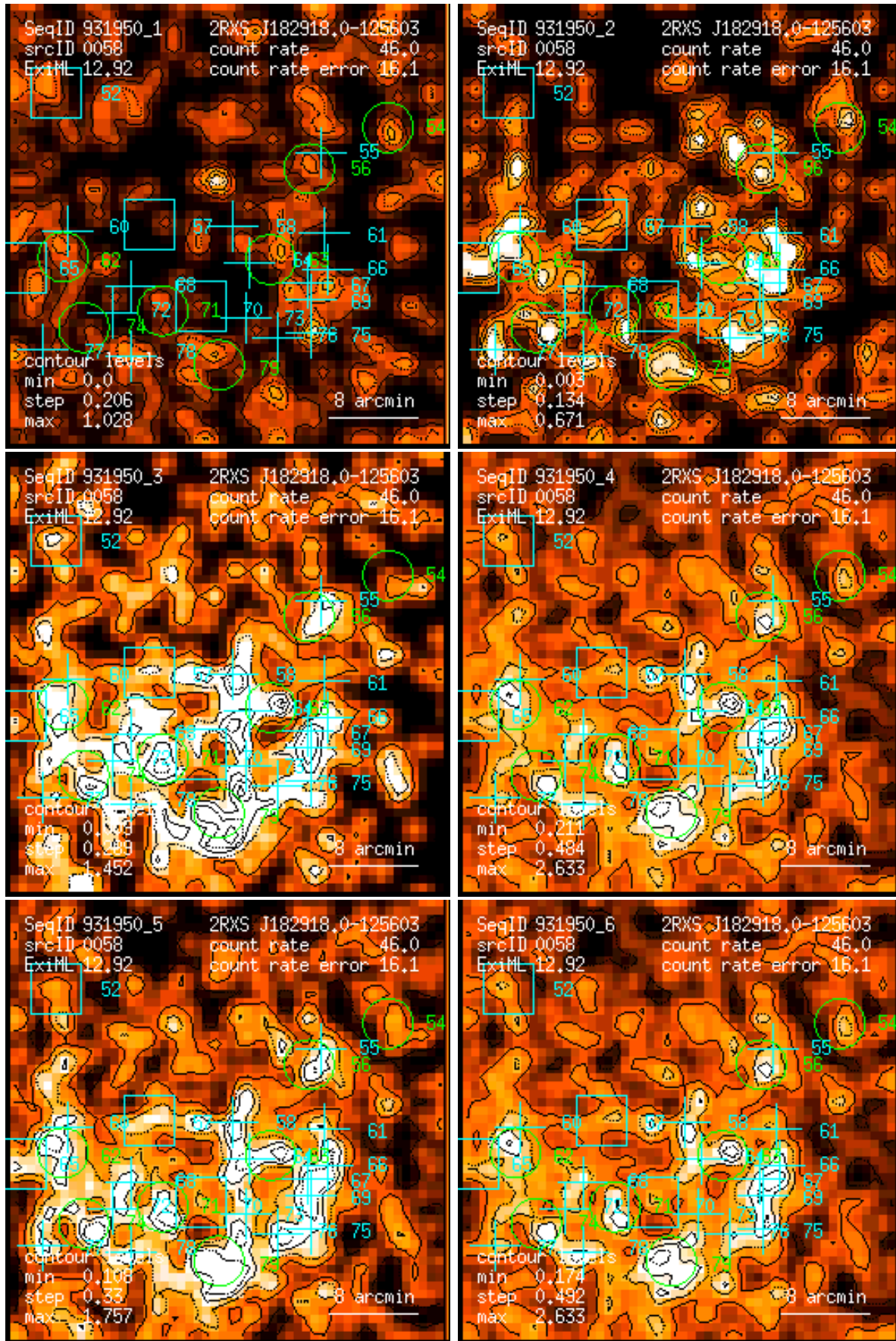
Figure 58: RASS 931950: detection 0058: band rate images, Gaussian filter: (1) PSPC channels 11 – 41, (2) 52 – 90, (3) 91 – 201, (4) 11 – 235, (5) 52 – 201, (6) 11 – 201. Broad band rates in counts/ks. Band rate contour levels in counts/ks/arcmin 2 .
