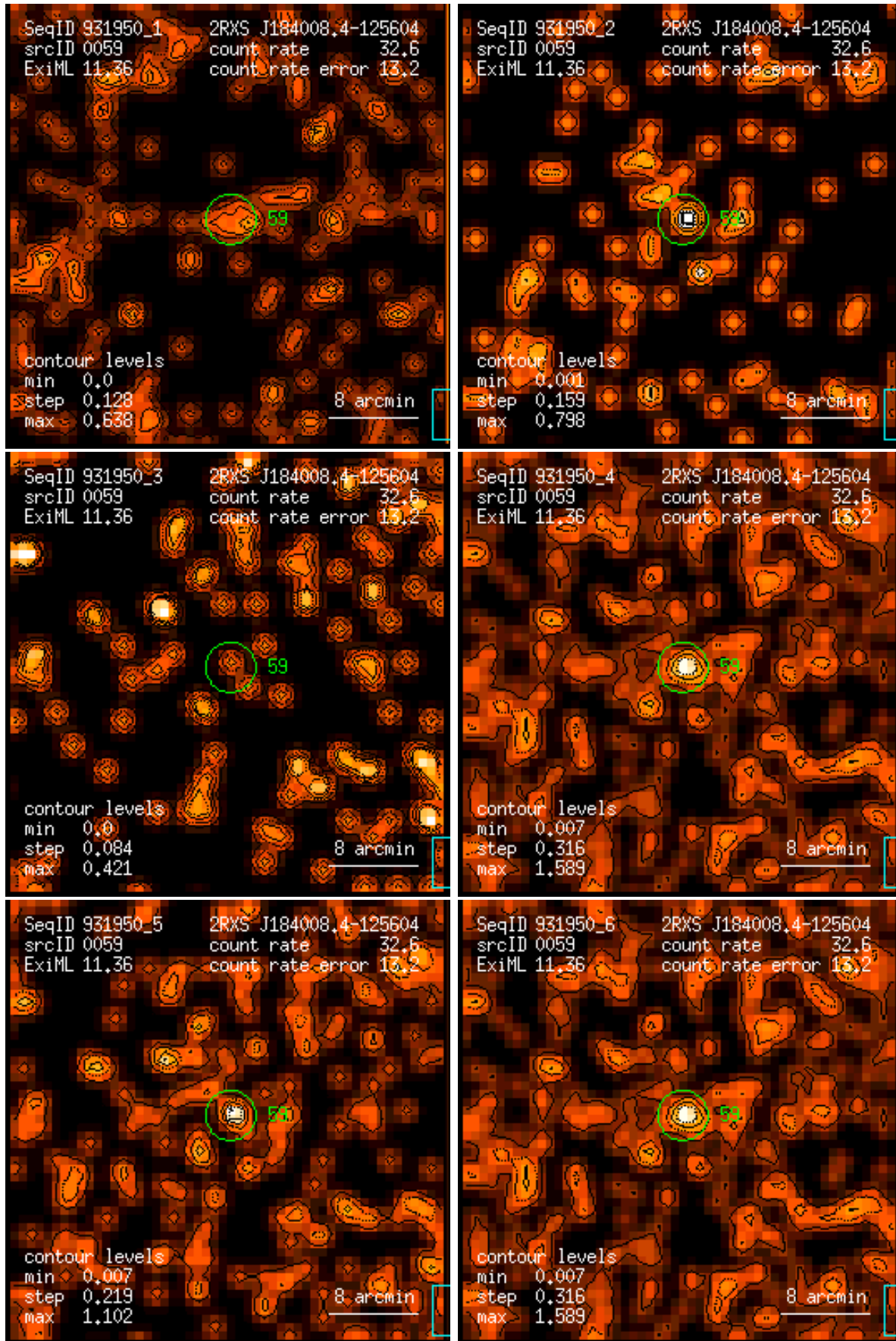
Figure 59: RASS 931950: detection 0059: band rate images, Gaussian filter: (1) PSPC channels 11 – 41, (2) 52 – 90, (3) 91 – 201, (4) 11 – 235, (5) 52 – 201, (6) 11 – 201. Broad band rates in counts/ks. Band rate contour levels in counts/ks/arcmin 2 .
