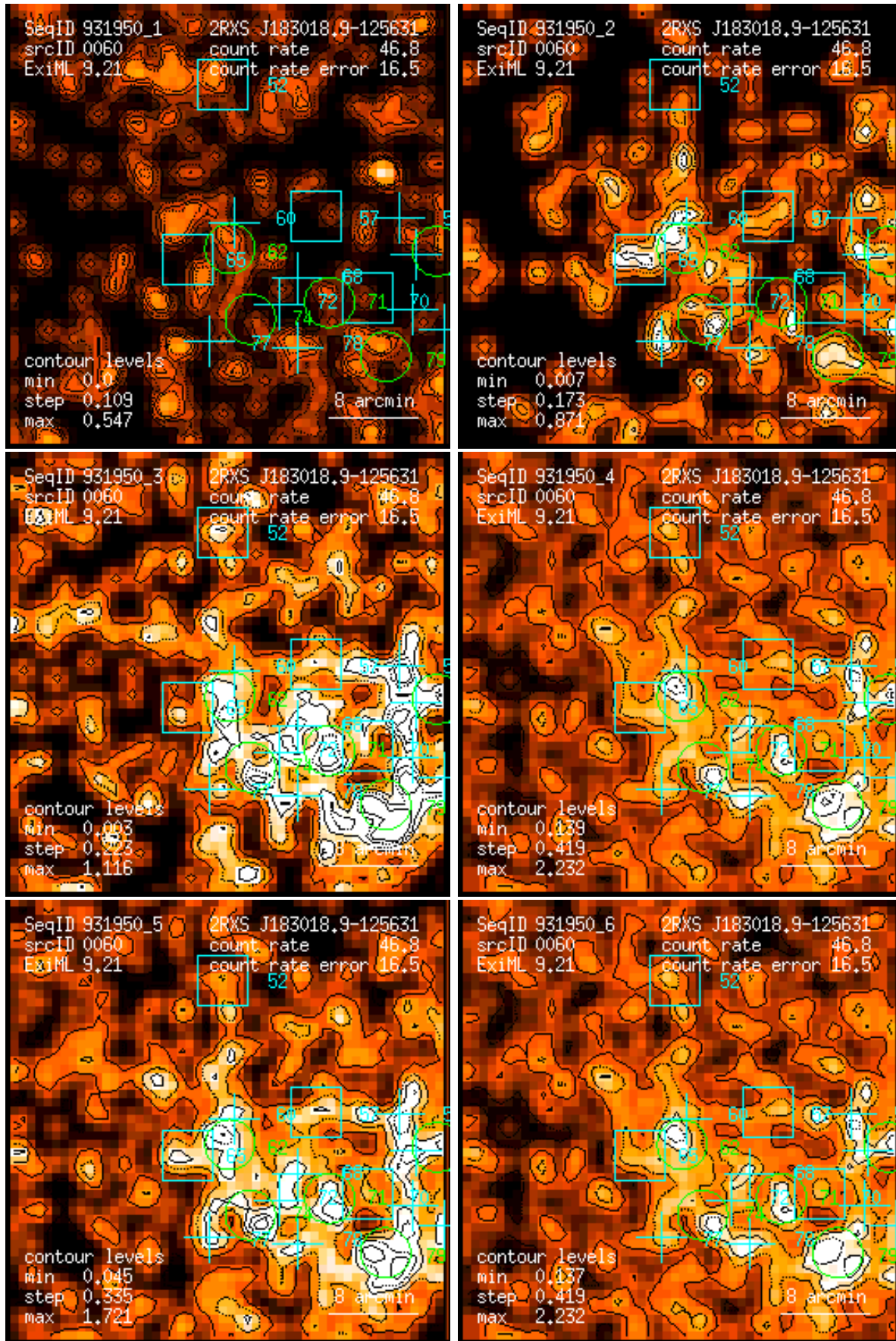
Figure 60: RASS 931950: detection 0060: band rate images, Gaussian filter: (1) PSPC channels 11 – 41, (2) 52 – 90, (3) 91 – 201, (4) 11 – 235, (5) 52 – 201, (6) 11 – 201. Broad band rates in counts/ks. Band rate contour levels in counts/ks/arcmin 2 .
