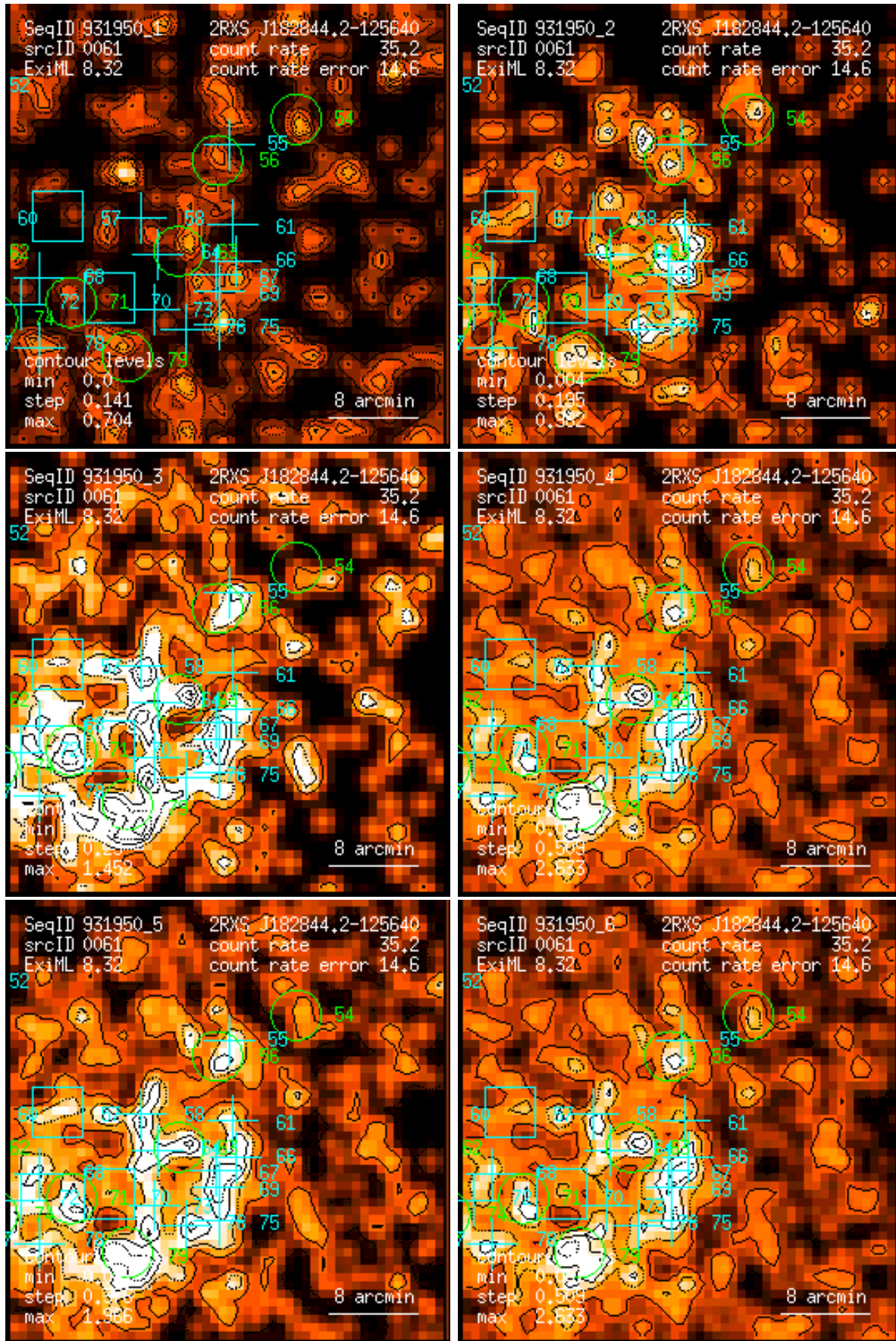
Figure 61: RASS 931950: detection 0061: band rate images, Gaussian filter: (1) PSPC channels 11 – 41, (2) 52 – 90, (3) 91 – 201, (4) 11 – 235, (5) 52 – 201, (6) 11 – 201. Broad band rates in counts/ks. Band rate contour levels in counts/ks/arcmin 2 .
