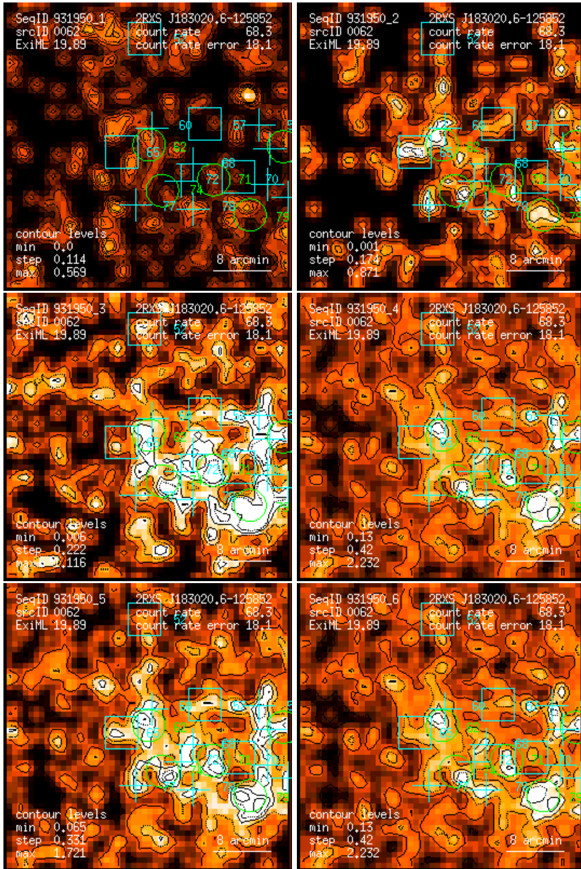
Figure 62: RASS 931950: detection 0062: band rate images, Gaussian filter: (1) PSPC channels 11 – 41, (2) 52 – 90, (3) 91 – 201, (4) 11 – 235, (5) 52 – 201, (6) 11 – 201. Broad band rates in counts/ks. Band rate contour levels in counts/ks/arcmin 2 .
