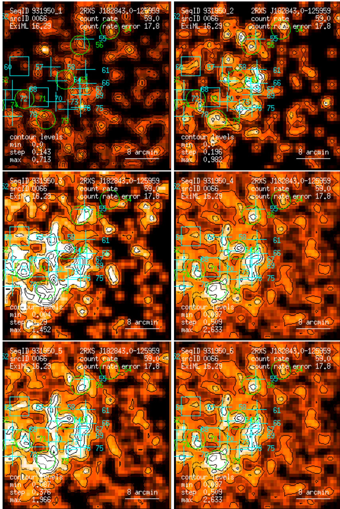
Figure 66: RASS 931950: detection 0066: band rate images, Gaussian filter: (1) PSPC channels 11 – 41, (2) 52 – 90, (3) 91 – 201, (4) 11 – 235, (5) 52 – 201, (6) 11 – 201. Broad band rates in counts/ks. Band rate contour levels in counts/ks/arcmin 2 .
