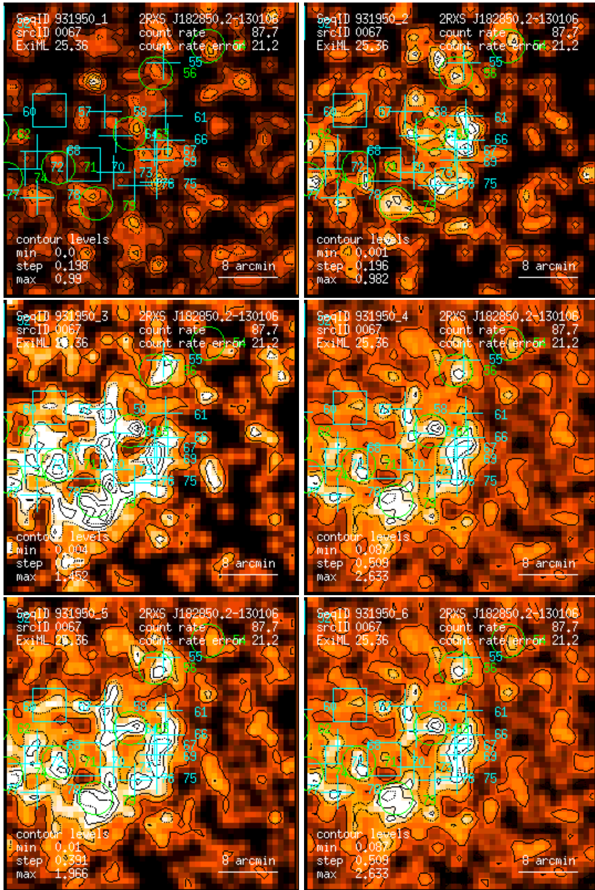
Figure 67: RASS 931950: detection 0067: band rate images, Gaussian filter: (1) PSPC channels 11 – 41, (2) 52 – 90, (3) 91 – 201, (4) 11 – 235, (5) 52 – 201, (6) 11 – 201. Broad band rates in counts/ks. Band rate contour levels in counts/ks/arcmin 2 .
