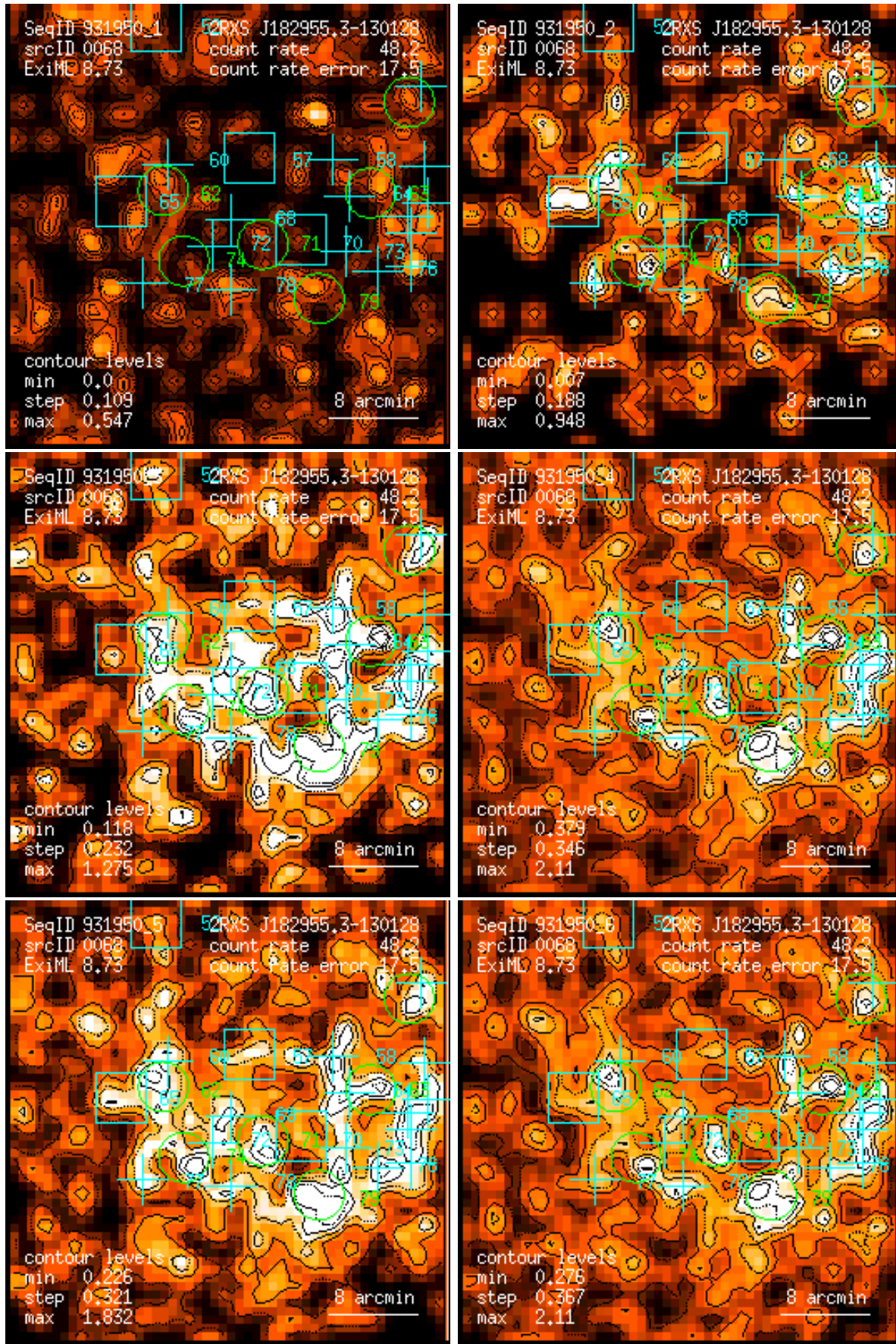
Figure 68: RASS 931950: detection 0068: band rate images, Gaussian filter: (1) PSPC channels 11 – 41, (2) 52 – 90, (3) 91 – 201, (4) 11 – 235, (5) 52 – 201, (6) 11 – 201. Broad band rates in counts/ks. Band rate contour levels in counts/ks/arcmin 2 .
