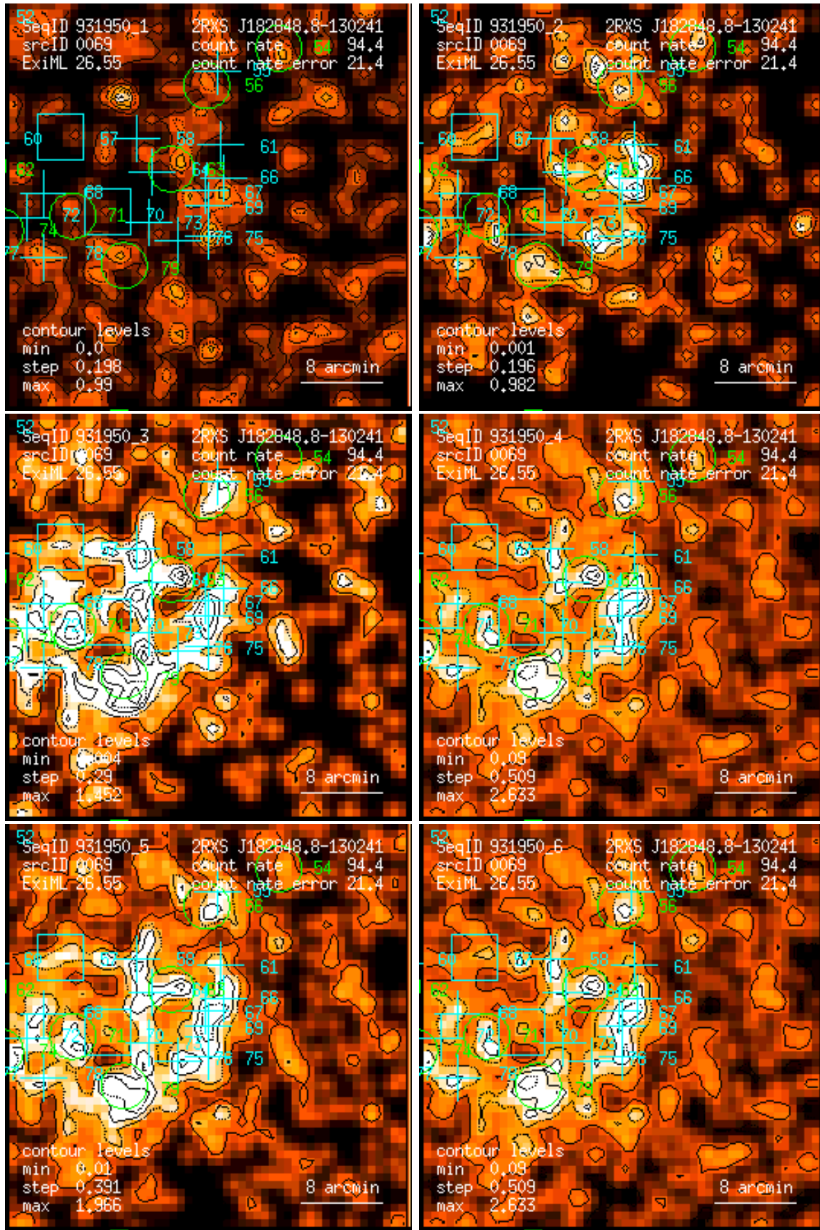
Figure 69: RASS 931950: detection 0069: band rate images, Gaussian filter: (1) PSPC channels 11 – 41, (2) 52 – 90, (3) 91 – 201, (4) 11 – 235, (5) 52 – 201, (6) 11 – 201. Broad band rates in counts/ks. Band rate contour levels in counts/ks/arcmin 2 .
