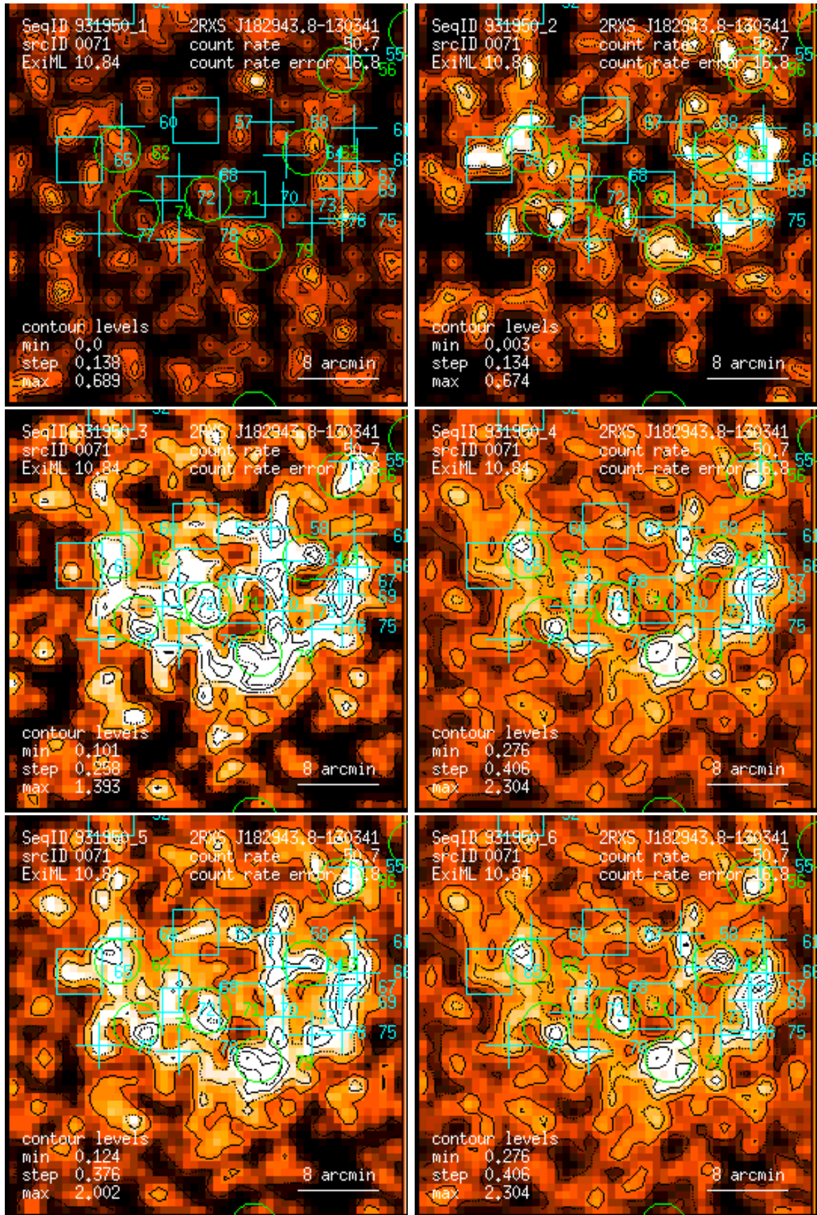
Figure 71: RASS 931950: detection 0071: band rate images, Gaussian filter: (1) PSPC channels 11 – 41, (2) 52 – 90, (3) 91 – 201, (4) 11 – 235, (5) 52 – 201, (6) 11 – 201. Broad band rates in counts/ks. Band rate contour levels in counts/ks/arcmin 2 .
